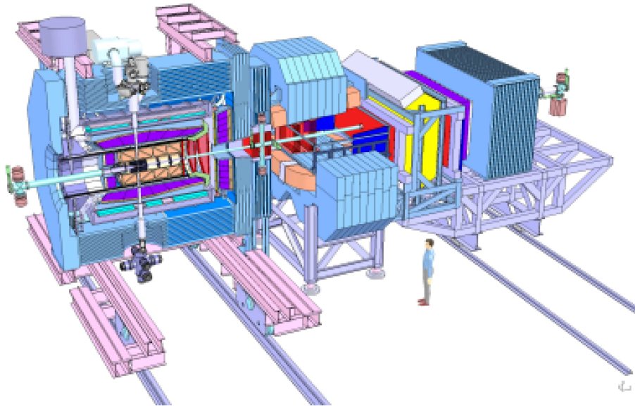
Fig. 1. 3D-view of the \bar{P} ANDA detector.
