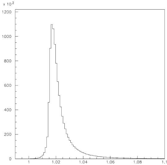
Fig. 9. Radiative correction in Eq. (22).
