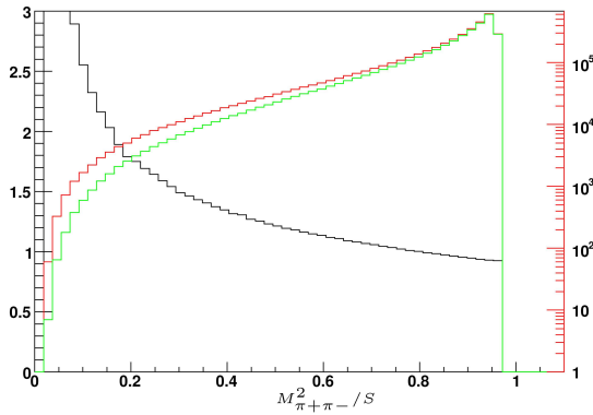
Fig. 3. Comparison of result using \sum_{\lambda,\epsilon} |M_I|^2 (green line) with that using matrix element taken from Ref. [7] (red line). Black line represents their ratio.
