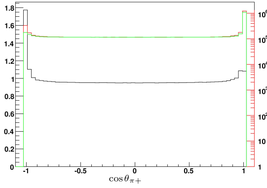
Fig. 6. Comparison of result using \sum_{\lambda,\epsilon} |M'_I|^2 (green line) with that using matrix element taken from Ref. [7] (red line). Black line represents their ratio.
