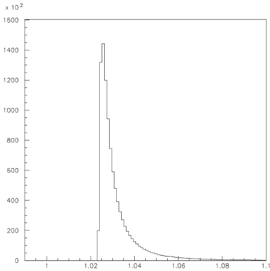
Fig. 8. Coulomb correction from Ref. [10].
