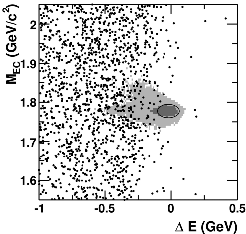
Fig. 3. The \Delta E - M_{\text{EC}} plot for the \tau^- \rightarrow e^- \gamma search in BABAR. The data are shown as dots while contours that would contain 90% and 50% of any signal, as determined by Monte Carlo simulations, are shown as the light- and dark-shaded regions. The ellipse indicates the 2\sigma region for a signal. It can be seen that there are no events within the 2\sigma ellipse.
