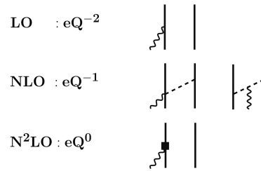
Fig. 1. Diagrams illustrating one- and two-body currents up to N^2LO ( eQ^0 ). Nucleons, pions, and photons are denoted by solid, dashed, and wavy lines, respectively. The square represents the relativistic correction to the LO one-body current. Only one among the possible time orderings is shown for the NLO diagrams.
