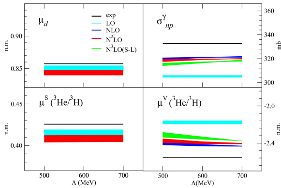
Fig. 3. (color online). Cumulative LO , NLO , N^2LO , and N^3LO(S-L) contributions for the deuteron and trinucleon isoscalar and isovector magnetic moments, and np radiative capture.
