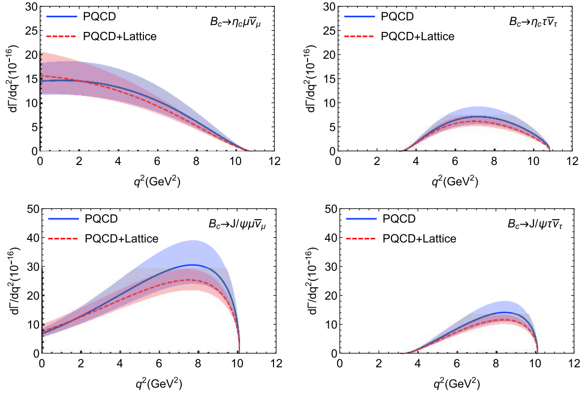
Fig. 4. (color online) Theoretical predictions of the q^2 dependence of d\Gamma/dq^2 for the decays B_c \rightarrow (\eta_c, J/\psi)l\bar{\nu}_l in the PQCD and “PQCD+Lattice” approaches. The bands show the theoretical uncertainties.
