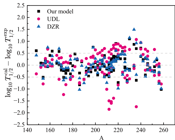
Fig. 4. (color online) Same as Fig. 2 but for odd-odd nuclei.
