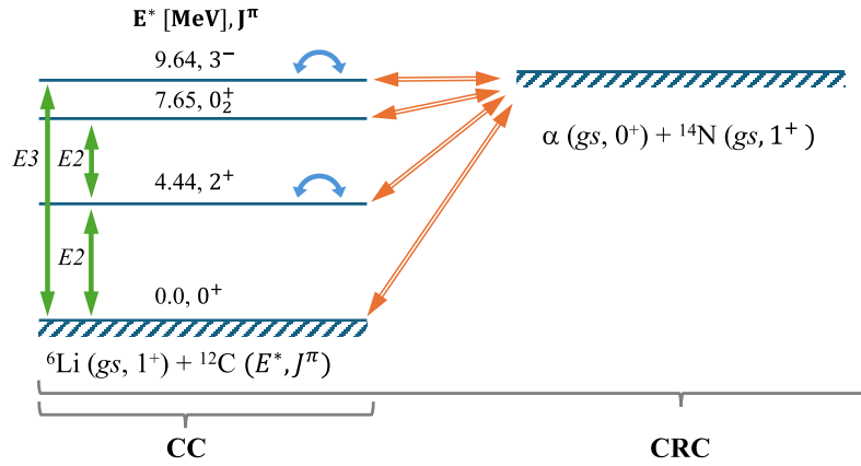
Fig. 5. (color online) Coupling scheme used in the CC calculations for {}^{12}\text{C}({}^6\text{Li}, {}^6\text{Li}){}^{12}\text{C}^* inelastic scattering and in the CRC calculations for {}^{12}\text{C}({}^6\text{Li}, \alpha){}^{14}\text{N} . Double-headed arrows indicate E\lambda transitions, backward-pointing arrows indicate spin-reorientation, and double-lined arrows indicate reaction transitions.
