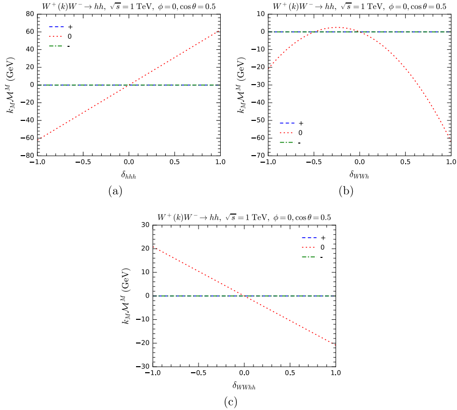
Fig. 14. (color online) k_M \mathcal{M}^M for WW \rightarrow hh as a function of anomalous overall couplings \delta_{hhh} (a), \delta_{WW h} (b), and \delta_{WW hh} (c). Various helicity configurations are shown.
