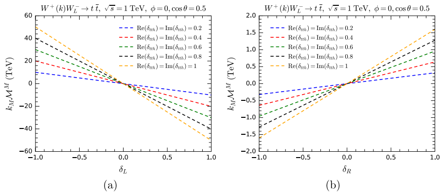
Fig. 17. (color online) k_M \mathcal{M}^M for WW \rightarrow t\bar{t} as a function of \delta_L (a) and \delta_R (b) with different values of \text{Re}(\delta_{tth}) and \text{Im}(\delta_{tth}) , serving as a test for gauge symmetry in the presence of the SMEFT operator \mathcal{O}_{t\Phi} .
