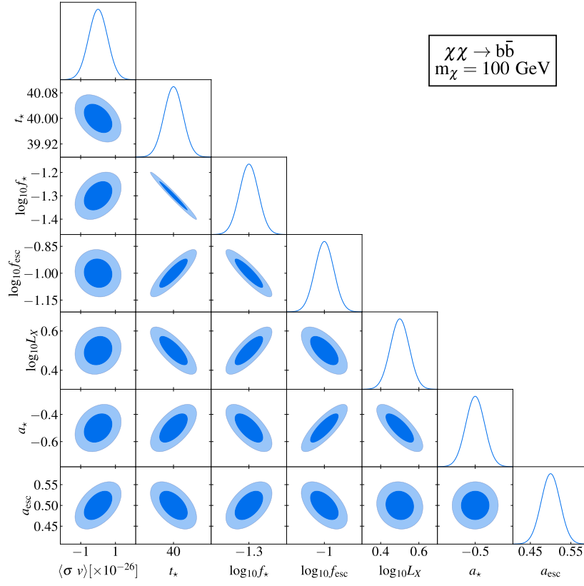
Fig. A2. Same as Fig. A1 but for 100 GeV DM particles annihilating into bottom-anti-bottom quark pairs.
