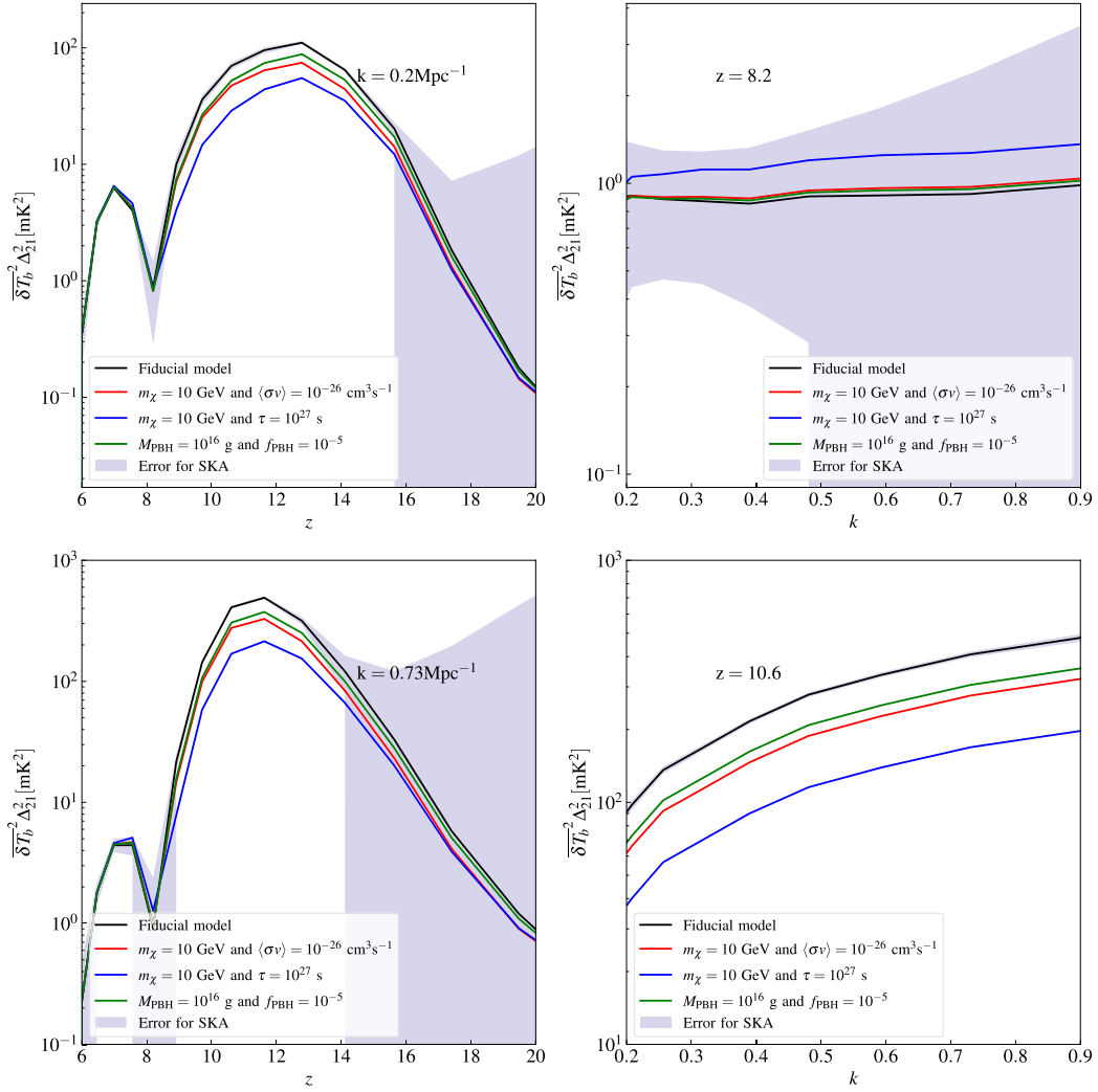
Fig. 2. (color online) 21 cm power spectrum under different energy injection scenarios. Left-hand panels: 21 cm power spectrum as a function of redshift z at fixed scales k = 0.2 \text{ Mpc}^{-1} and k = 0.73 \text{ Mpc}^{-1} . Right-hand panels: 21 cm power spectrum as a function of the scale at redshift z = 8.2 and z = 10.6 . In each panel, the instrumental noise is shown by the shaded region. Black curves show the 21 cm power spectrum of the fiducial model. Red curves show 21 cm power spectrum with DM particle annihilation through \chi\chi \rightarrow e^+e^- channel with m_\chi = 10 \text{ GeV} and \langle\sigma v\rangle = 10^{-26} \text{ cm}^3 \text{ s}^{-1} . Blue curves show 21 cm power spectrum with DM particle decay through \chi \rightarrow e^+e^- channel with m_\chi = 10 \text{ GeV} and \tau = 10^{27} \text{ s} . Green curves show 21 cm power spectrum with PBH Hawking radiation, with M_{\text{PBH}} = 10^{16} \text{ g} and f_{\text{PBH}} = 10^{-5} .
