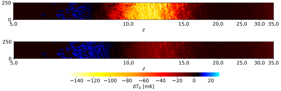
Fig. 1. (color online) Lightcone slices of the differential brightness temperature in our (250 \text{ Mpc})^3 large simulation box. The fiducial model is shown on the upper panel. The bottom panel shows the slice with DM particle decay through \chi \rightarrow e^+e^- channel with m_\chi = 10 \text{ GeV} and \tau = 10^{27} \text{ s} .
