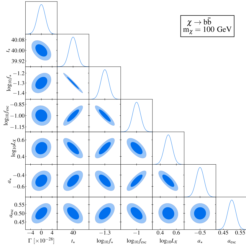
Fig. A4. Same as Fig. A1 but for 100 GeV DM particles decaying into bottom-anti-bottom quark pairs.
