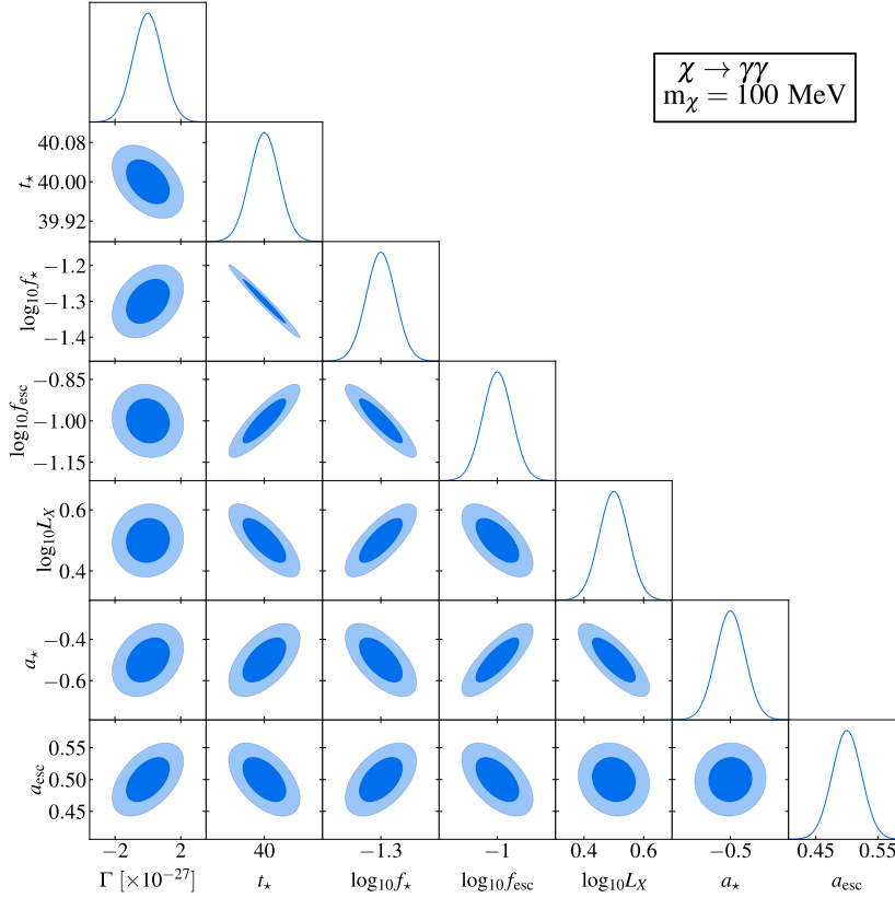
Fig. A3. Same as Fig. A1 but for 100 MeV DM particles decaying into photon pairs.
