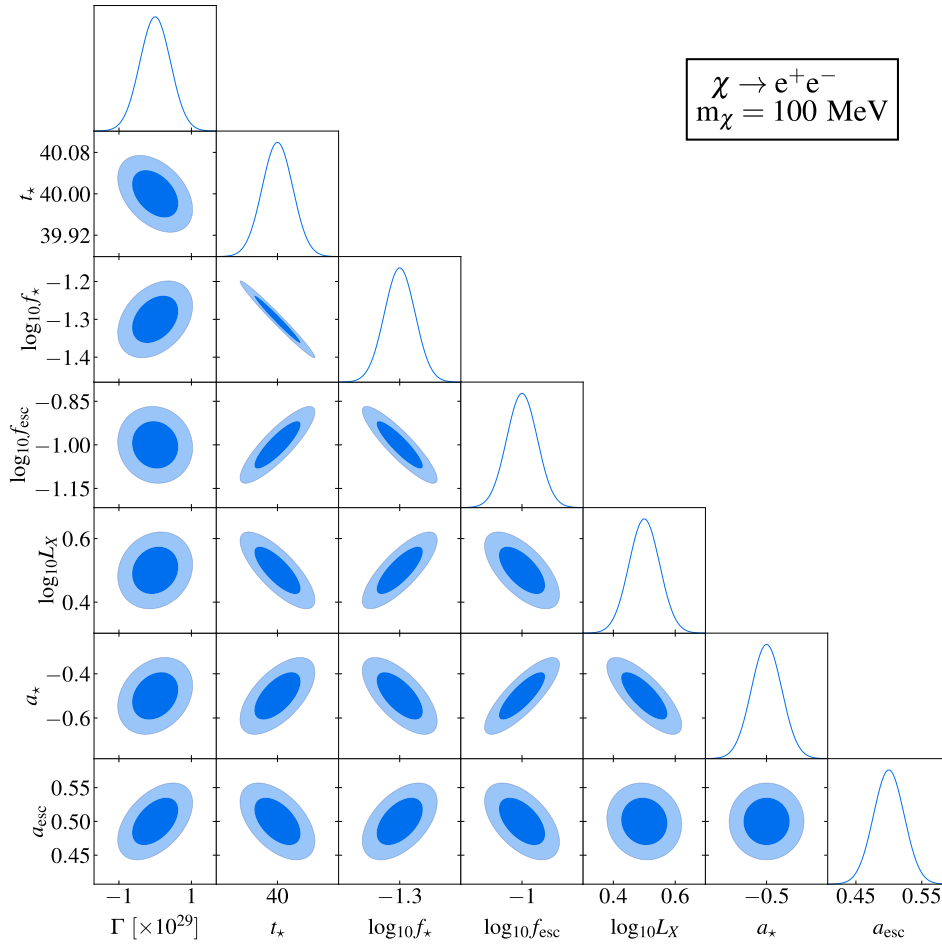
Fig. 5. (color online) Fisher forecast for probing DM decay through the \chi \rightarrow e^+e^- channel using the 21 cm power spectrum by the SKA. 1\sigma and 2\sigma confidence intervals are represented by dark and light shaded areas, respectively, with solid curves indicating the marginalized posteriors. The fiducial model used is consistent with that shown in Fig. 2. The assumed DM particle mass is m_\chi = 100 MeV, integrated over 10,000 h.
