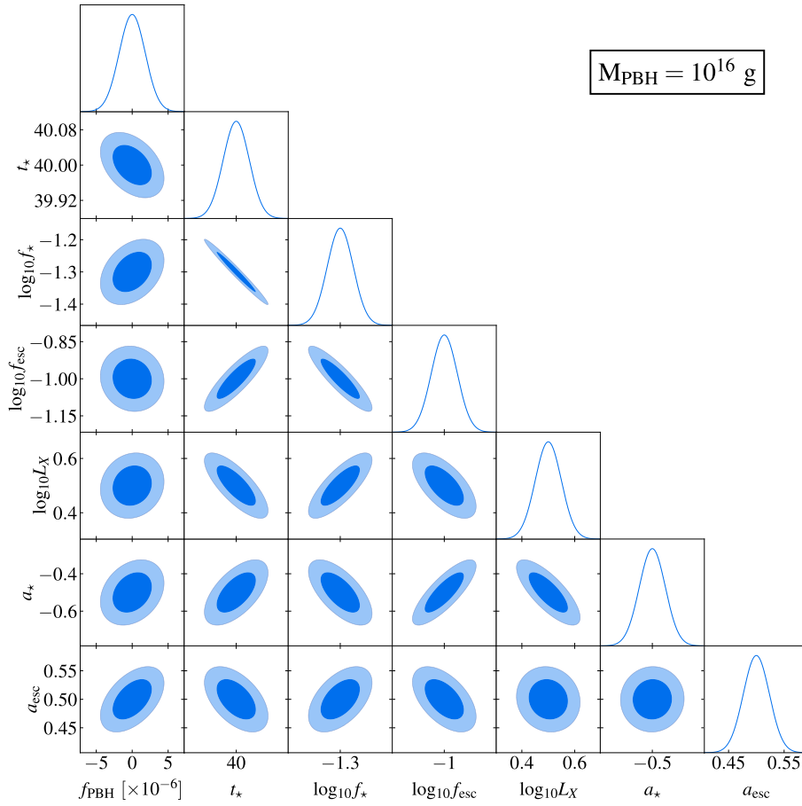
Fig. 7. (color online) Fisher forecast for probing PBH Hawking radiation using the 21 cm power spectrum by the SKA. Dark and light shaded regions correspond to contours at 1\sigma and 2\sigma confidence intervals, respectively. Solid curves represent the marginalized posteriors of the model parameters. The fiducial model used is consistent with that shown in Fig. 2. The mass of PBH is assumed to be M_{\text{PBH}} = 10^{16} g with an integration duration of 10,000 h.
