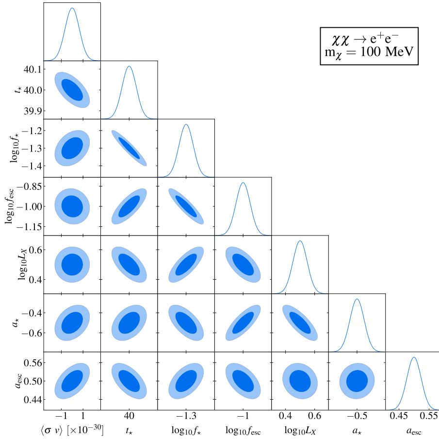
Fig. 3. (color online) Fisher forecast for probing DM annihilation through the \chi\chi \rightarrow e^+e^- channel using the 21 cm power spectrum via the SKA. 1\sigma and 2\sigma confidence intervals are represented by dark and light shaded areas, respectively, with solid curves indicating the marginalized posteriors. The fiducial model used is consistent with that shown in Fig. 2. The assumed DM particle mass is m_\chi = 100 MeV, integrated over 10,000 h.
