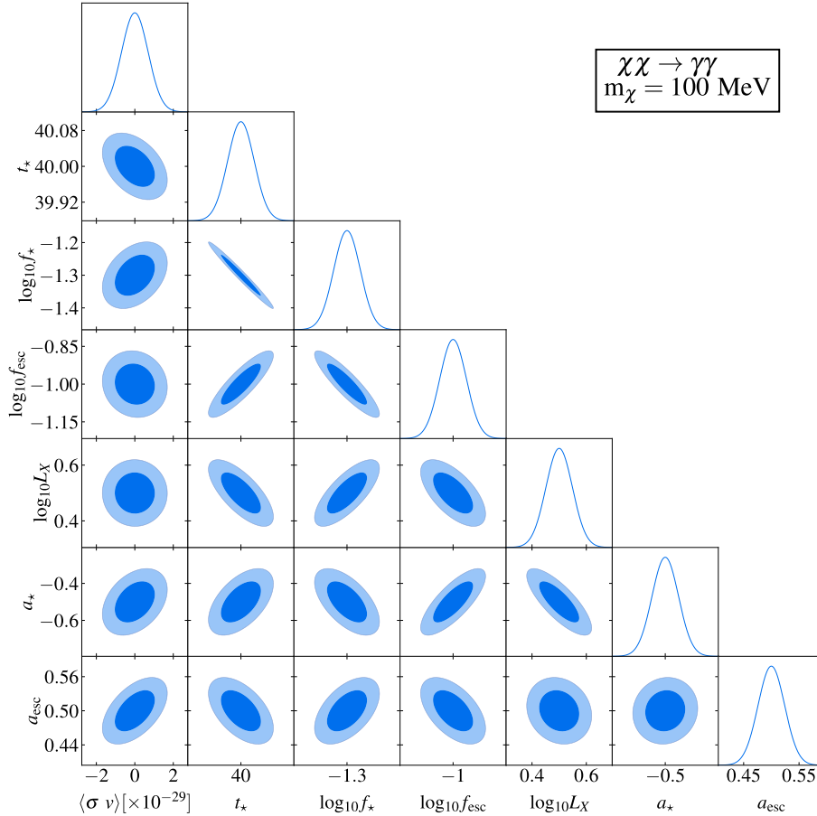
Fig. A1. Fisher forecast for probing DM annihilation through the \chi\chi \rightarrow \gamma\gamma channel using 21 cm power spectrum by the SKA. 1\sigma and 2\sigma confidence intervals are represented by dark and light shaded areas, respectively, with solid curves indicating the marginalized posteriors. Fiducial model used is consistent with that shown in Fig. 2. The assumed DM particle mass is m_\chi = 100 MeV, integrated over 10,000 h.
