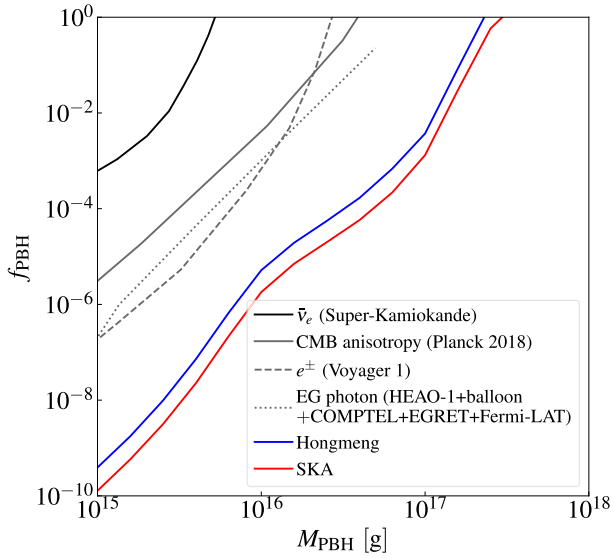
Fig. 8. (color online) Prospective sensitivity of the SKA for probing the PBHs. The 1\sigma confidence-level sensitivity of the SKA project to measure the abundance of PBHs within the mass range of 10^{15} - 10^{18} g is shown by the red curve. For comparison, we show the existing upper limits at the 2\sigma confidence level from observations of the diffusion neutrino background (black curve) [46], CMB anisotropies (gray solid curve) [31, 32, 34], extra-galactic photons (gray dotted curve) [54], and electron-positron pairs (gray dashed curve) [47]. The prospective sensitivity of the 21 cm global signal (blue curve) is also considered.
