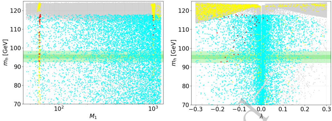
Fig. 6. (color online) The scanning results using the parameter ranges in Table 2 are shown. The left panel displays the relationship between the light scalar Higgs boson mass m_h and M_1 , while the right panel presents the correlation between m_h and \lambda . The color scheme follows the description in the color conditions and the surrounding context. The green band indicates that m_h = 95.4 \pm 1 GeV, the light green area represents m_h = 95.4 \pm 3 GeV.
