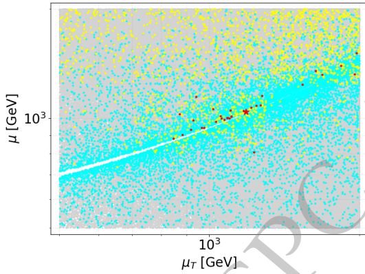
Fig. 7. (color online) The results of the global scan are presented in the \mu - \mu_T plane. The parameter points follow the color scheme described in the text. Red star markers represent parameter sets satisfying all red point conditions plus the Higgs mass constraint m_h = 95.4 \pm 1 GeV.
