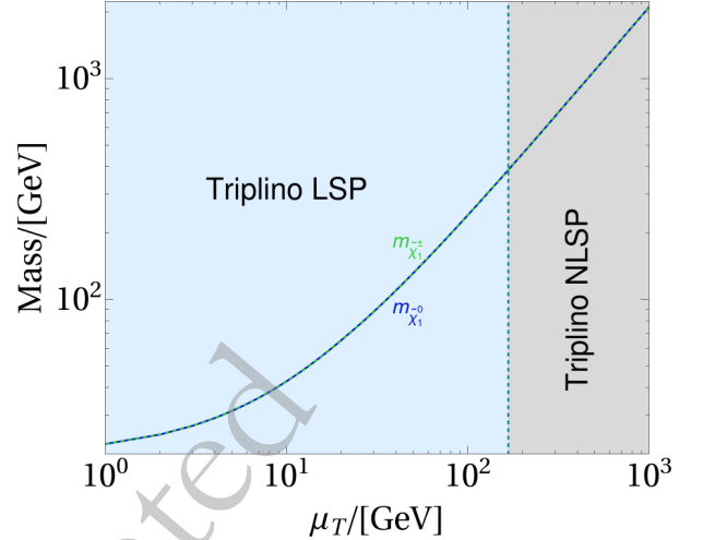
Fig. 5. (color online) The masses of the charged triplino and neutral triplino as a function of \mu_T , and the status for the LSP.
