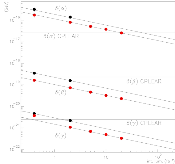
Fig. 2. Limits on the CPT violating parameters \alpha , \beta and \gamma obtainable by KLOE-2 as a function of the integrated luminosity. See the text for details.
