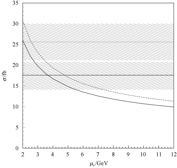
Fig. 1. The cross section as a function of the \mu_r at \sqrt{s}=10.58\text{ GeV} . The dashed and solid curves are the cross sections in the m_c=1.4 and m_c=1.5 respectively. The above and under reseau bands represent the measured cross sections by the Belle and BABAR experiments, with respective systematic and statistical errors.
