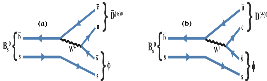
Fig. 1. (color online) Feynman diagrams for (a) B_s^0 \rightarrow \bar{D}^{*0} \phi and (b) B_s^0 \rightarrow D^{*0} \phi decays.
