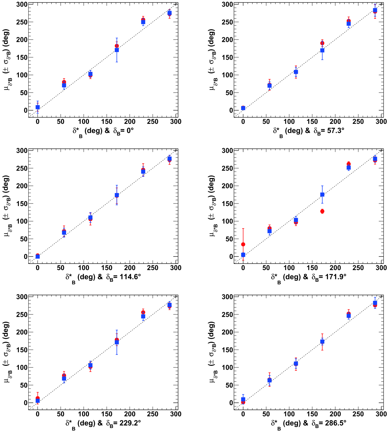
Fig. A4. (color online) Fitted mean values of \delta_B^* ( \mu_{\delta_B^*} ), for r_B^{(*)} = 0.22 (red circles) and 0.4 (blue squares) as a function of \delta_B^* for initial true value of \gamma of 65.66^\circ (1.146 rad). In each figure, the dashed black line indicates the initial \delta_B^* true value, and the displayed uncertainties are the fitted resolutions on \delta_B^* ( i.e. \sigma_{\delta_B^*} ).
