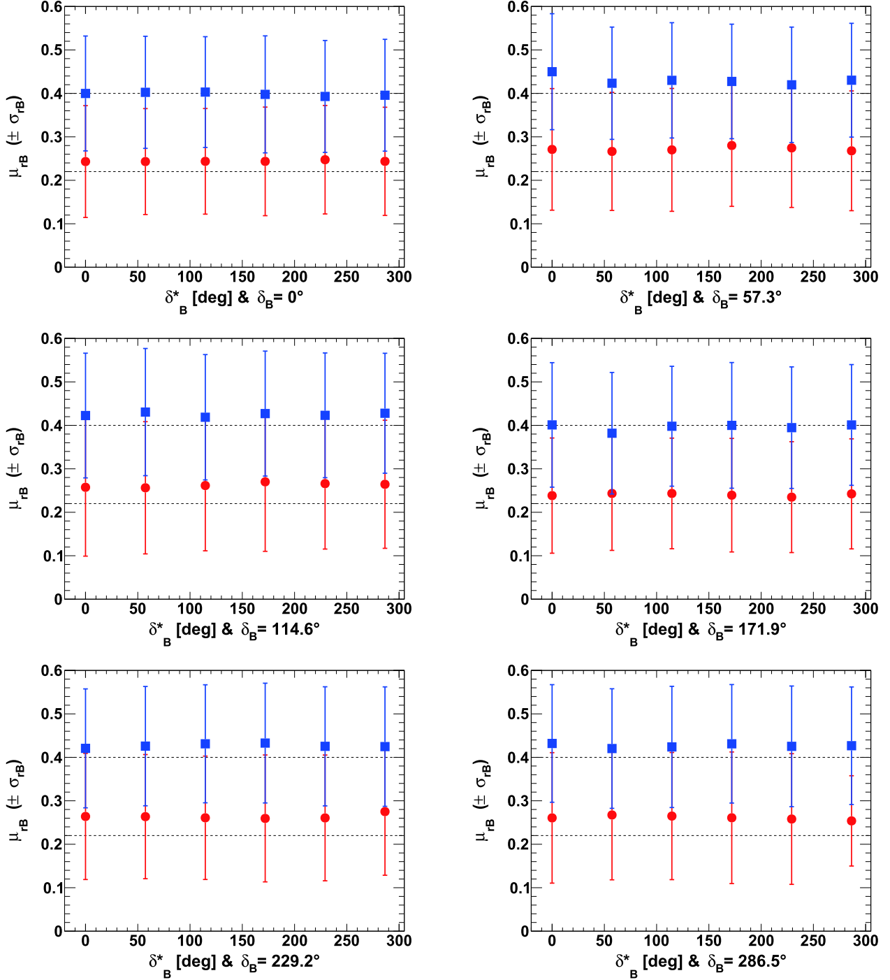
Fig. A1. (color online) Fitted mean values of r_B ( \mu_{r_B} ), for r_B^{(*)} = 0.22 (red circles) and 0.4 (blue squares) as a function of \delta_B^{(*)} for initial true value of \gamma of 65.66^\circ ( 1.146 rad). In each figure, the horizontal dashed black line indicates the initial r_B true value, and the displayed uncertainties are the fitted resolutions on r_B ( i.e. \sigma_{r_B} ).
