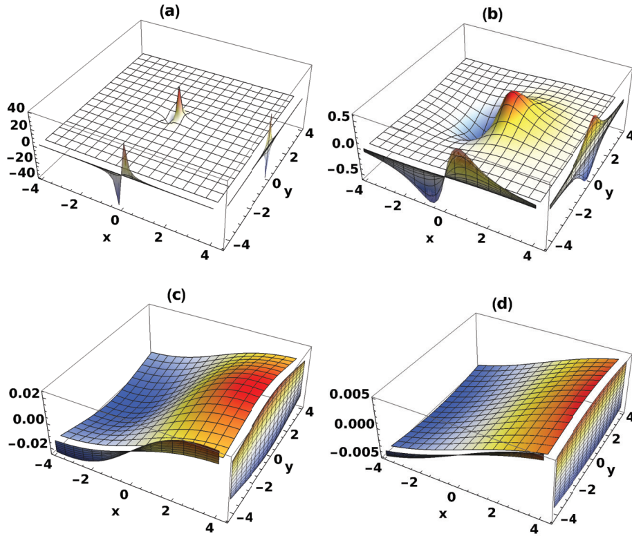
Fig. 4. (color online) Space distribution of the magnetic field B_y on x - y plane with z=0 in Fig. 4(a), z=1/\gamma (fm) in Fig. 4(b), z=5/\gamma (fm) in Fig. 4(c), and z=10/\gamma (fm) in Fig. 4(d) produced by a single proton with 100 GeV traveling through the +z direction, calculated within the point-like model.
