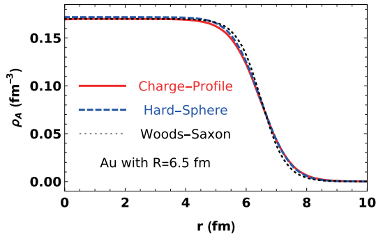
Fig. 7. (color online) Charge density in the nucleus from the convolution of the Woods-Saxon nucleon distribution with three charge densities in a nucleon for Au with R = 6.5 fm.
