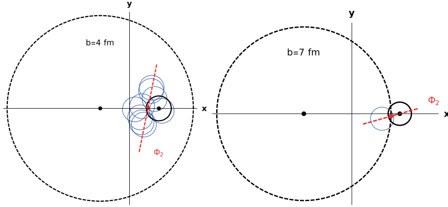
Fig. 10. (color online) Examples of participant distributions in one event for b = 4 fm (left panel), and b = 7 fm (right panel). The red point is the center of mass r_c , and the red line indicates \Phi_2 . The blue circles are participants from the target nucleus, while the black circle is the single projectile proton.
