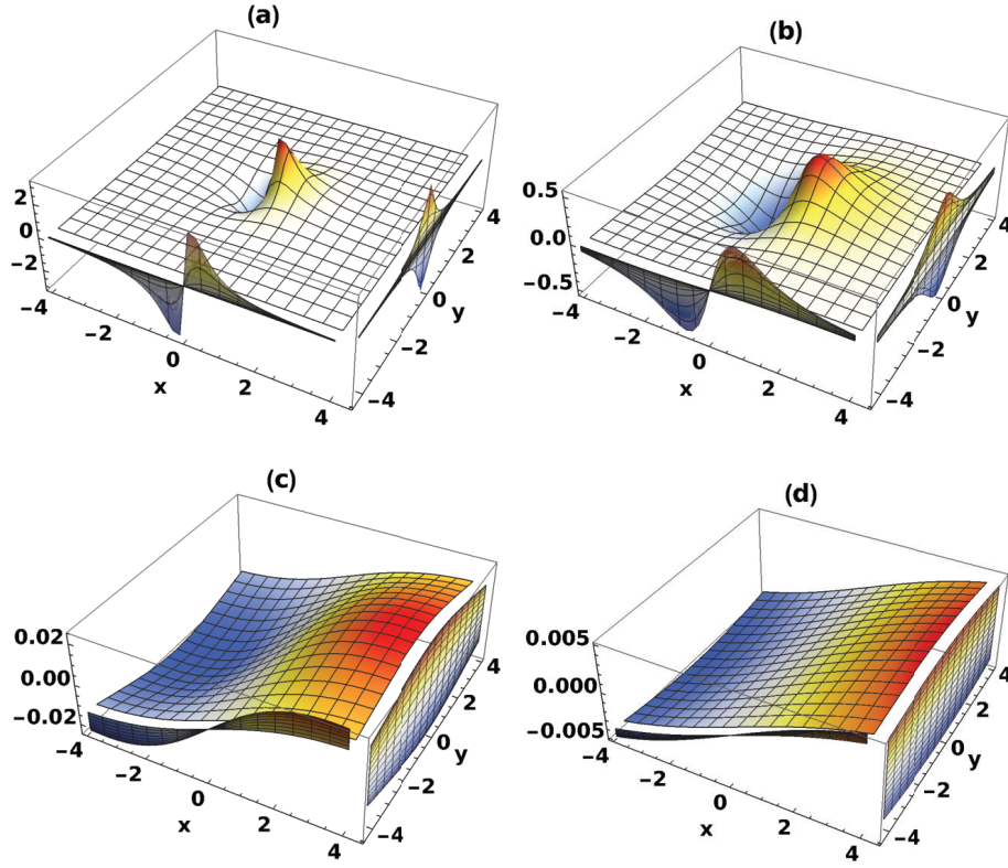
Fig. 3. (color online) Space distribution of magnetic field B_y on the x - y plane with z=0 in Fig. 3(a), z=1/\gamma (fm) in Fig. 3(b), z=5/\gamma (fm) in Fig. 3(c), and z=10/\gamma (fm) in Fig. 3(d) produced by a single proton with 100 GeV traveling through the +z direction, calculated within the Charge-Profile model.
