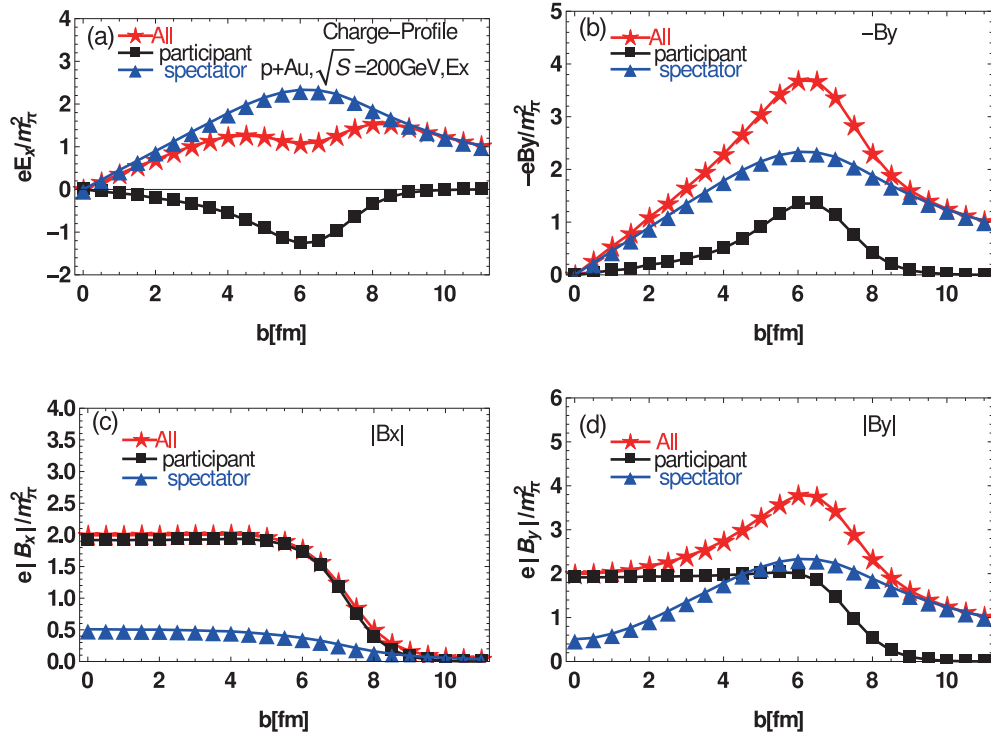
Fig. 11. (color online) Electromagnetic fields at t=0 and r = r_c as functions of the impact parameter b with the charge-orofile model.
