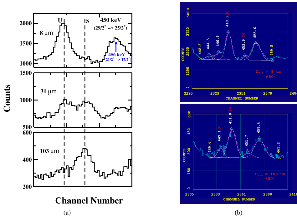
Fig. 10. (color online) A portion of energy spectrum showing the shifted (S) and unshifted (U) peaks of 450 keV \gamma -ray transition of yrast band in ^{177}\text{Re} at three different target–stopper distances ( D_{T-S} ) and (b) A portion of energy spectrum showing the fitting of unshifted energy (U) of 450 keV (our peaks of interest) at D_{T-S} = 8 \mu\text{m} (first distance) and D_{T-S} = 103 \mu\text{m} (distance of minimum intensity). Data are obtained with detectors at 50^\circ relative to the beam direction. (* The \gamma -ray energy peak marked in blue corresponds to the \gamma -ray transition belonging to Band 2 [6].)
