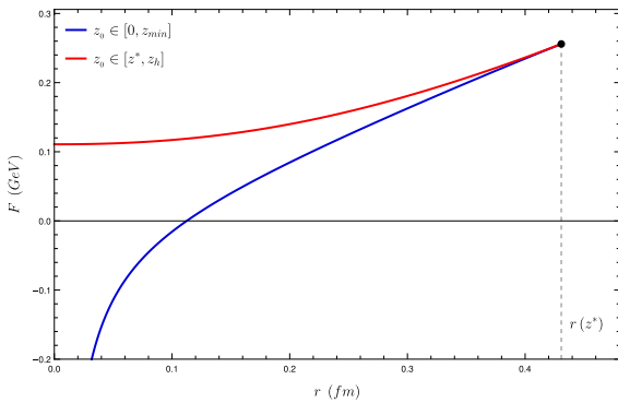
Fig. 9. (color online) Free energy as a function of quark distance at T = 1.01T_d .
