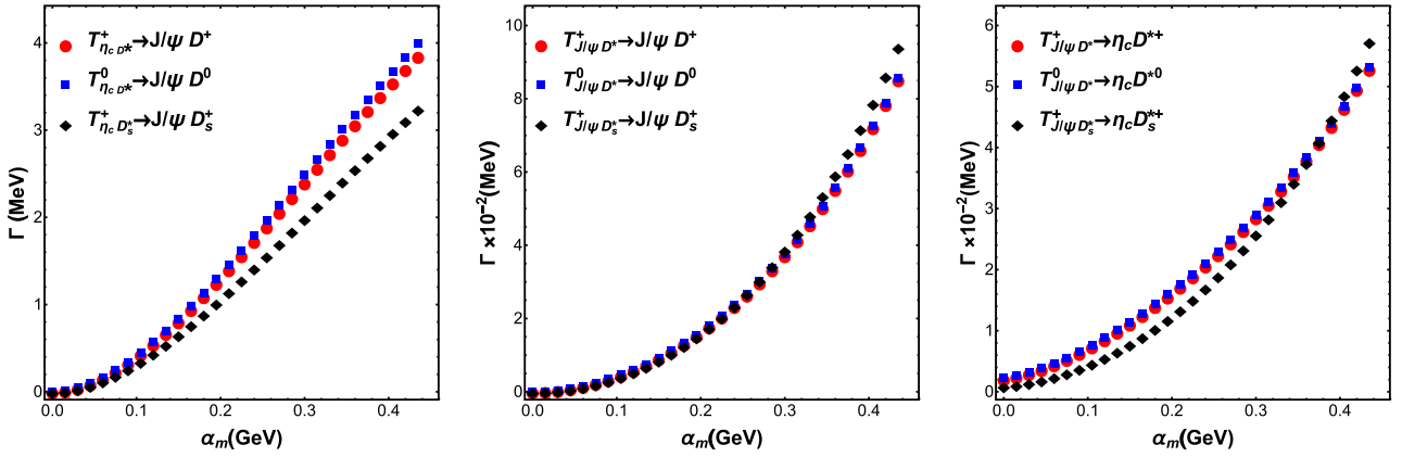
Fig. 4. (color online) At the binding energy \varepsilon = 5 MeV, the two-body decay widths of T_{cc\bar{c}\bar{q}} vary with the scale parameter \alpha_m (GeV). The panels correspond to the decays T_{\eta_c D^*}^+ \rightarrow J/\psi D (left), T_{J/\psi D^*}^+ \rightarrow J/\psi D (middle), and T_{J/\psi D^*}^+ \rightarrow \eta_c D^* (right).
