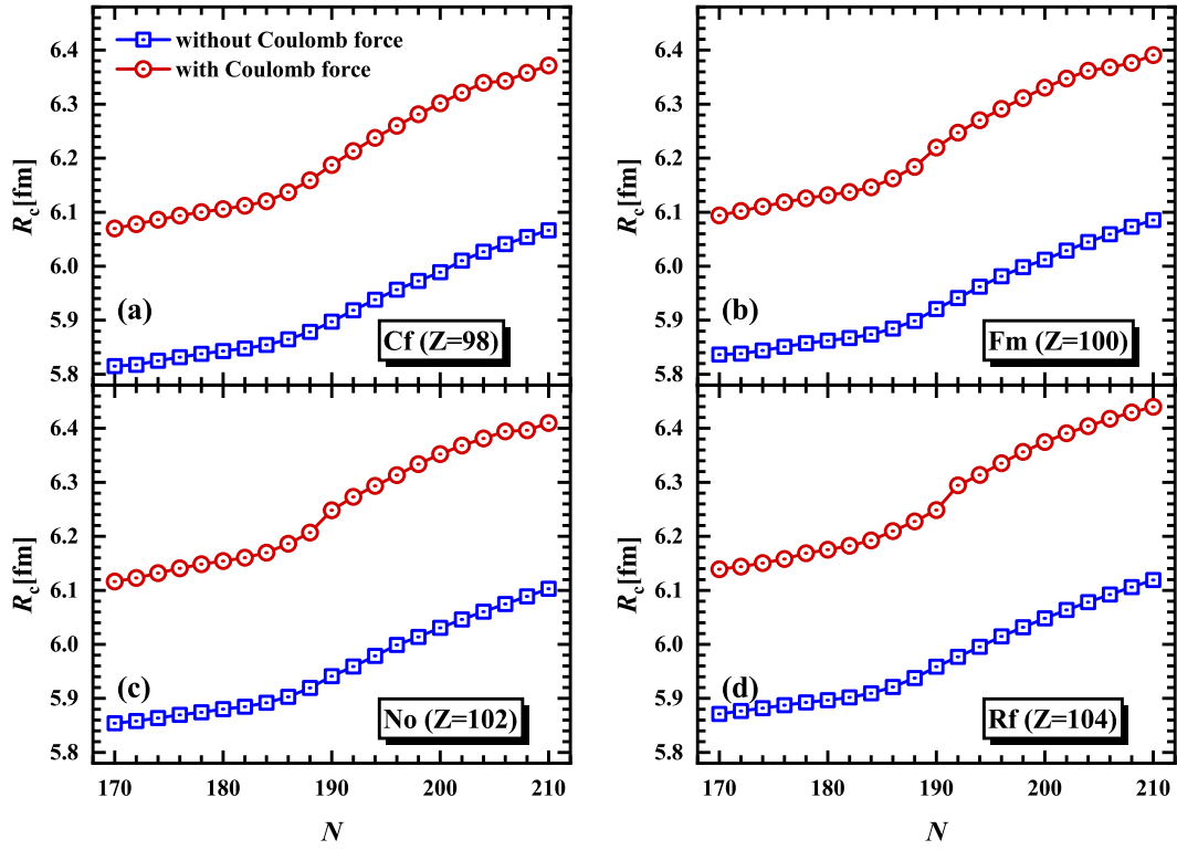
Fig. 14. (color online) Same as the caption of Fig. 9, but for the charge radius R_c .
