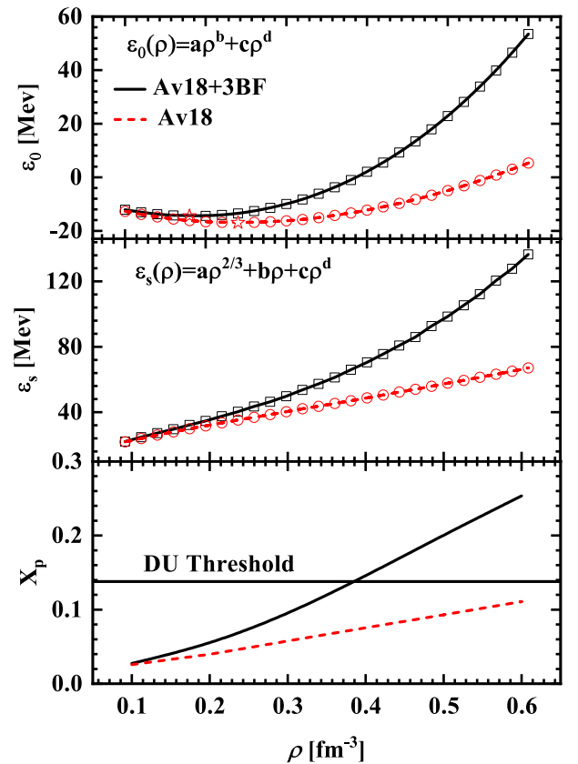
Fig. 1. (color online) Binding energy per nucleon of symmetric nuclear matter \varepsilon_0(\rho) (upper panel), nuclear symmetry energy \varepsilon_s (middle panel), and proton fraction of \beta -stable matter (lower panel) at zero temperature as functions of nucleon density. The black open squares and red open circles represent the results obtained with Av18 + 3BF and Av18 only, respectively. The black solid and red short-dashed lines in the upper and middle panels denote the corresponding fits obtained from Eq. (52). The red stars indicate the saturation points obtained from the BHF calculations. In the lower panel, the black solid and red short-dashed lines correspond to the results obtained with Av18 + 3BF and Av18 only, respectively. The horizontal line indicates the threshold proton fraction for the direct Urca (DU) neutrino emission process.
