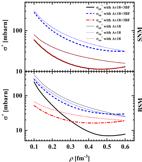
Fig. 3. (color online) Effective total cross sections, \sigma^* , as functions of density for symmetric nuclear matter (upper panel) and \beta -stable nuclear matter (lower panel). The black solid, blue short-dashed, and red short-dash-dotted lines denote the proton–proton and neutron–proton scattering results. The thick and thin lines indicate the results obtained with Av18 + 3BF and Av18 only, respectively.
