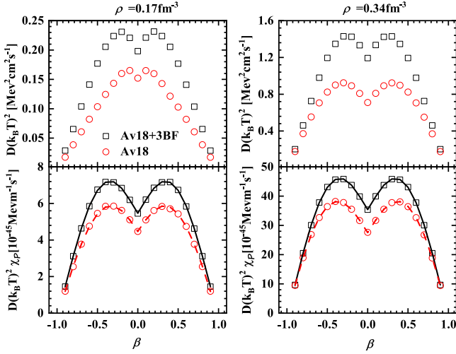
Fig. 5. (color online) Isospin dependence of the diffusion coefficient D (upper panel) and D\chi_P (lower panel) at densities of 0.17 \text{ fm}^{-3} and 0.34 \text{ fm}^{-3} . The black open squares and red open circles represent the results obtained using Av18 + 3BF and Av18 alone, respectively. The black solid and red short-dashed lines in the lower panel denote the corresponding fits obtained from Eq. (54).
