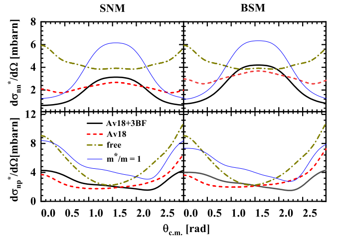
Fig. 2. (color online) Differential cross sections as functions of the center-of-mass (c.m.) scattering angle at a density of \rho = 0.35 \text{ fm}^{-3} and a c.m. energy of E_{\text{c.m.}} = 75 \text{ MeV} . The left (right) panels correspond to symmetric nuclear matter ( \beta -stable nuclear matter), whereas the upper (lower) panels show the neutron-neutron (neutron-proton) channel. The thick solid, thick short-dashed, and thick short-dash-dotted lines denote the results obtained with Av18 + 3BF, Av18 only, and in free space, respectively. The thin solid lines show the results calculated from Eq. (38) using Av18 + 3BF with m^*/m = 1 .
