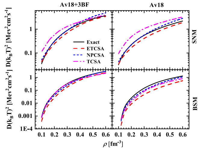
Fig. 4. (color online) Isospin diffusion coefficients obtained under different approximations in symmetric and \beta -stable nuclear matter. The black solid, red dashed, blue short-dashed, and magenta dash-dotted lines denote the exact result, the effective total cross-section approximation (ETCSA), the neutron–proton cross-section approximation (NPCSA), and the total cross-section approximation (TCSA), respectively.
