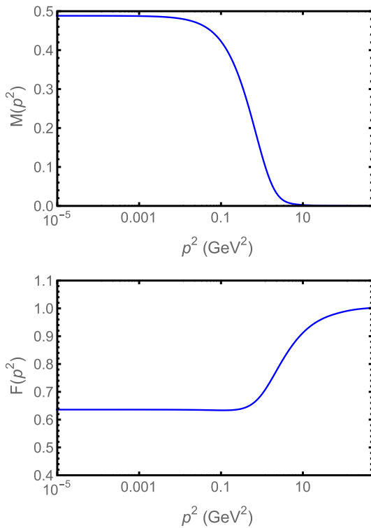
Fig. 2. (color online) Behavior of the dressed-quark mass function M(p^2) and wave-function renormalization F(p^2) for the RGZ-model truncation of the SDE in the chiral limit. These plots show that the dressed-quark mass decreases as the momentum increases. In the low-momentum region, p^2 < 1 ( M(0) \approx 0.5 GeV), the dressed mass is large because of dynamical chiral symmetry breaking. Conversely, at large momentum, p^2 \gg 1 , the dressed-quark mass vanishes in the chirally symmetric state. In this limit, the quark wave-function renormalization F(p^2) approaches unity.
