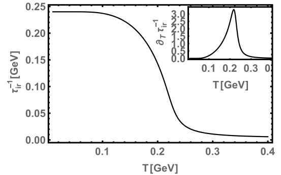
Fig. 17. Temperature dependence of the confinement scale \tau_{ir}^{-1} for a finite current quark mass. A comparison with Fig. 16 shows that a physical quark mass smooths the transition; the peak in the thermal gradient is broader and lower, indicating that the phase transition becomes a continuous crossover.
