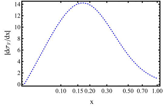
Fig. 12. (color online) Inflection-point analysis for the Lei–Chang model. The existence of a well-defined extremum (at x \approx 0.17 \text{ GeV}^2 ) confirms that the simplified model preserves the analytic structure indicative of a confined excitation, thereby supporting its validity for predicting hadron properties.
