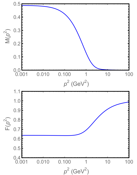
Fig. 3. (color online) The quark mass function M(p^2) and wave-function renormalization F(p^2) are shown for the Maris-Tandy (MT) model. These quantities illustrate the model's general behavior in the chiral limit, in which “gluon-cloud” dressing generates a large constituent-like mass from massless current quarks. This infrared behavior is a prerequisite for describing the observed hadron spectrum.
