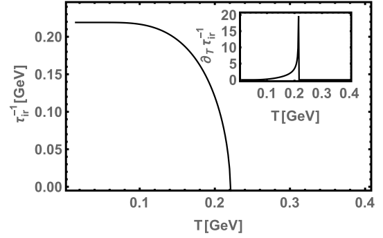
Fig. 16. The inverse confinement length scale \tau_{ir}^{-1} as a function of temperature T in the chiral limit. The main panel shows that the confinement scale decreases with increasing temperature. The inset shows the thermal derivative \partial_T \tau_{ir}^{-1} , whose sharp peak provides a precise definition of the critical temperature T_c for the deconfinement transition.
