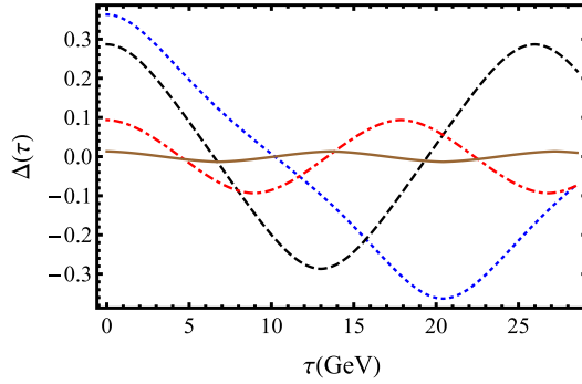
Fig. 14. (color online) \Delta(\tau) for various T as a function of \tau . The blue dotted curve is plotted at T = 0.07 \text{ GeV} , the black dashed curve at T = 0.11 \text{ GeV} , the red dot-dashed curve at T = 0.16 \text{ GeV} , and the solid brown curve at T = 0.21 \text{ GeV} . The Schwinger function oscillates, and the mass function has singularities; these features provide an unambiguous signal for the absence of a Lehmann representation and hence for confinement. As the temperature increases, no zero crossing occurs above a critical temperature T_c , thus indicating deconfinement.
