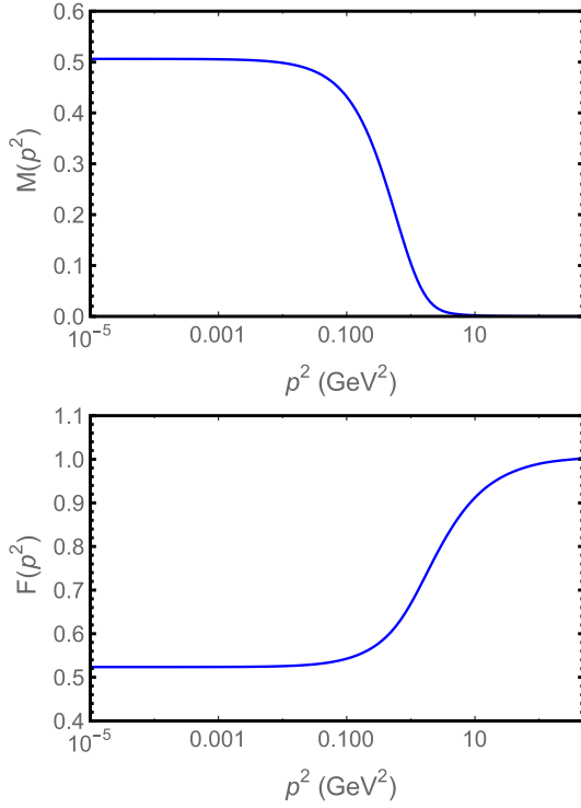
Fig. 5. (color online) The mass function M(p^2) and wave-function renormalization F(p^2) are shown for the Qin–Chang version of the MT model. This comparison highlights how different infrared saturation profiles affect the propagator. The stability of the infrared mass scale across models suggests that dynamical mass generation is a robust emergent feature of QCD, independent of specific truncation details.
