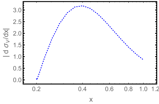
Fig. 13. (color online) This analysis examines the inflection point (at x \approx 0.37 \text{ GeV}^2 ) in the Qin–Chang model. Comparing this point with Fig. 11 shows how variations in the infrared kernel shift the confinement scale, providing a means of tuning model parameters using lattice QCD data.
