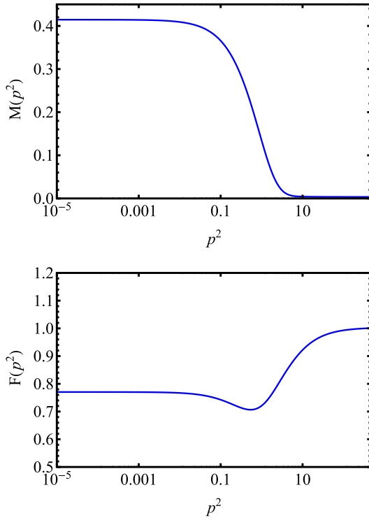
Fig. 4. (color online) Mass function M(p^2) and wavefunction renormalization F(p^2) for the Lei-Chang model. This figure shows that, even with a simplified interaction kernel, the SDE framework consistently yields the non-perturbative mass enhancement required to account for the majority of visible mass in the universe through hadronization.
