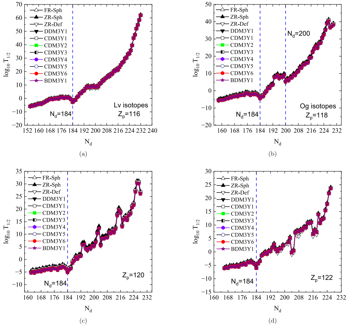
Fig. 4. (color online) Same as Fig. 3, but for superheavy isotopic chains: (a) Lv isotopes ( Z_p = 116 ), (b) Og isotopes ( Z_p = 118 ), (c) Z_p = 120 isotopes, and (d) Z_p = 122 isotopes. The vertical dashed lines denote the neutron shell closures at N_d = 184 and N_d = 200 .
