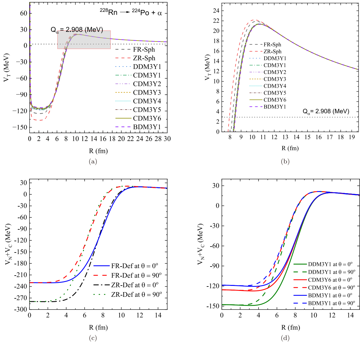
Fig. 1. (color online) The total \alpha -nucleus interaction potential, V_T , as a function of the separation distance R for the \alpha decay of ^{228}\text{Rn} \rightarrow ^{224}\text{Po} + \alpha , calculated using different M3Y-based effective interactions. (a) Full radial dependence of the total interaction potential, showing the nuclear pocket and the Coulomb barrier region. (b) Magnified view of the barrier region, highlighting the barrier height and position for each effective interaction. (c) Sum of the nuclear and Coulomb potentials, V_N + V_C , from deformed calculations using zero-range and finite-range exchange treatments at \theta = 0^\circ and 90^\circ . (d) Sum of the nuclear and Coulomb potentials, V_N + V_C , from deformed density-dependent interactions, including finite-range exchange effects, at \theta = 0^\circ and 90^\circ . The horizontal dotted line indicates the decay energy Q_\alpha = 2.908 MeV.
