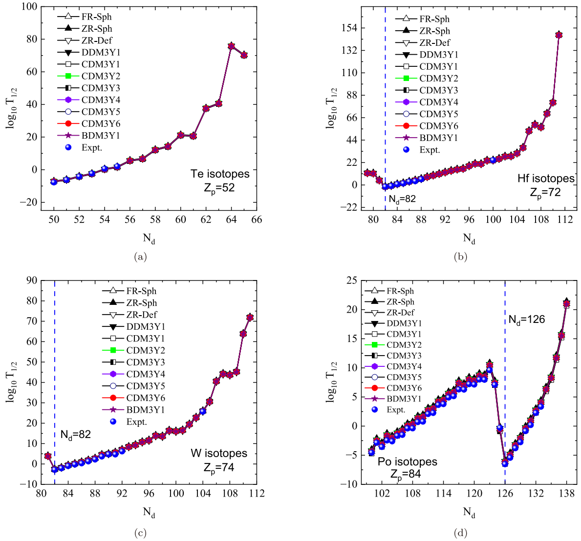
Fig. 3. (color online) The calculated and experimental logarithmic \alpha -decay half-lives, \log_{10} T_{1/2} (s), are plotted as a function of the neutron number of the daughter nucleus, N_d , for several isotopic chains. The theoretical results are obtained using different M3Y-based effective interactions. The panels correspond to (a) Te isotopes ( Z_p = 52 ), (b) Hf isotopes ( Z_p = 72 ), (c) W isotopes ( Z_p = 74 ), and (d) Po isotopes ( Z_p = 84 ). The vertical dashed lines indicate the neutron shell closures at N_d = 82 and N_d = 126 , highlighting the influence of shell effects on the \alpha -decay half-lives. Experimental data are shown for comparison.
