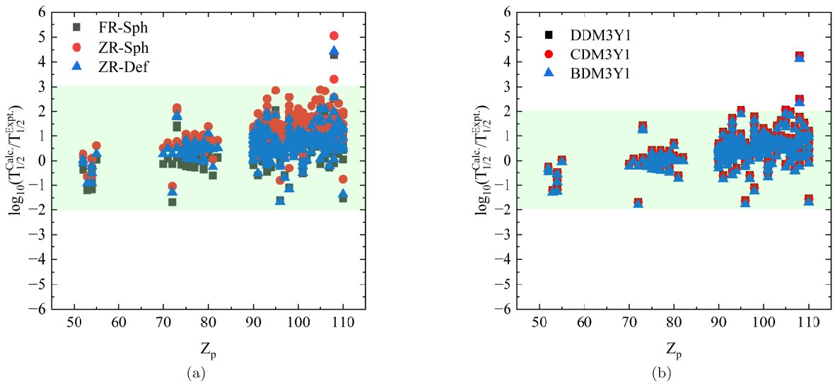
Fig. 2. (color online) Deviations between the calculated and experimental \alpha -decay half-lives, \log_{10}(T_{1/2}^{\text{Calc}}/T_{1/2}^{\text{Exp}}) , are plotted as a function of the atomic number of the parent nucleus, Z_p . The predictions are obtained using various M3Y-based effective interactions. Panel (a) shows the results for the FR-Sph, ZR-Sph, and ZR-Def interactions, while panel (b) presents those for the density-dependent interactions DDM3Y1, CDM3Y1, and BDM3Y1. The shaded region indicates deviations within \pm 2 orders of magnitude of the experimental half-lives.
