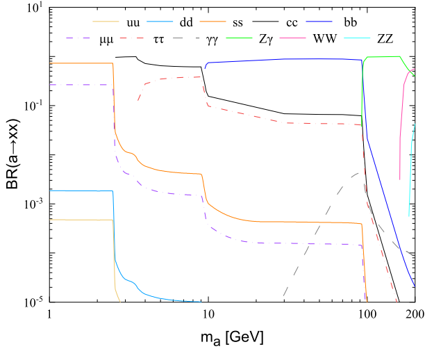
Fig. 1. (color online) Branching ratios for the different photophobic ALP decay modes as functions of the ALP mass m_a .
