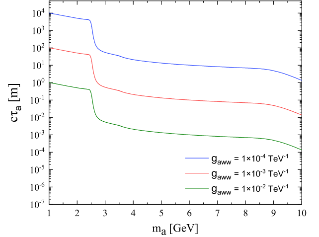
Fig. 2. (color online) The proper decay lengths of the ALP as functions of its mass, m_a , for several representative values of the coupling g_{aWW} .
