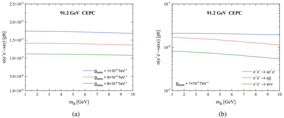
Fig. 4. (color online) Production cross sections for the processes e^+e^- \rightarrow a\gamma (a), av\bar{\nu} , ae^+e^- , and ajj (b) as functions of the ALP mass m_a for different values of the coupling g_{aWW} at the 91.2 GeV CEPC.
