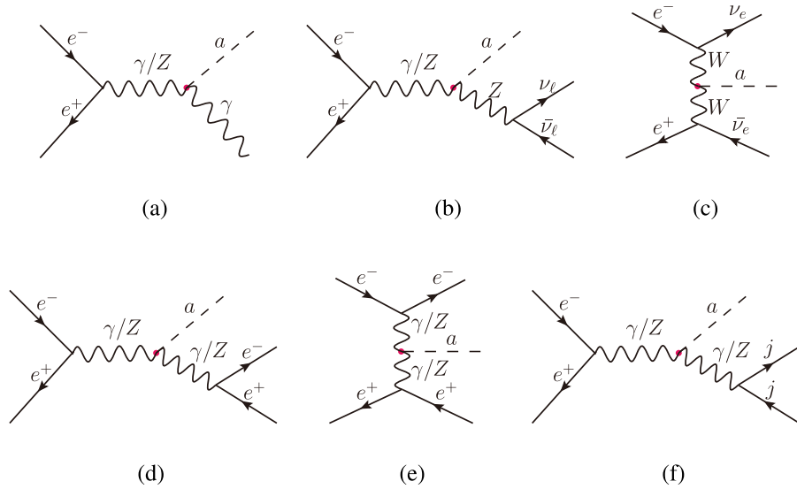
Fig. 3. (color online) Feynman diagrams for the single-production processes of the photophobic ALP: e^+e^- \rightarrow a\gamma (a), av\bar{\nu} (b,c), ae^+e^- (d,e), and ajj (f).
