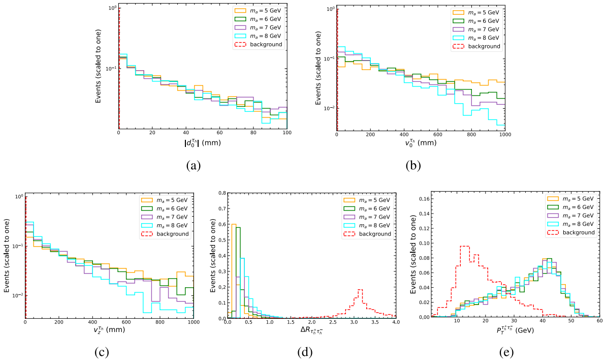
Fig. 10. (color online) Same as Fig. 7, but for the observables |d_0^{\tau h}| , v_0^{\tau h} , v_z^{\tau h} , \Delta R_{\tau_h^+\tau_h^-} , and P_T^{\tau_h^+\tau_h^-} with g_{aWW} = 1 \times 10^{-3} \text{TeV}^{-1} .
