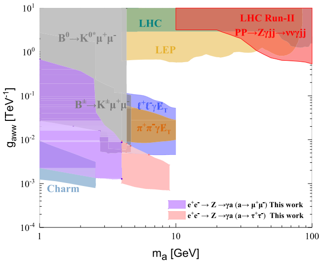
Fig. 11. (color online) Projected 95% C.L. sensitivities at the CEPC for light, long-lived photophobic ALPs in the \mu^+\mu^-\gamma (purple region) and \tau_h^+\tau_h^-\cancel{E}_T\gamma (pink region) channels, compared with other excluded regions.
