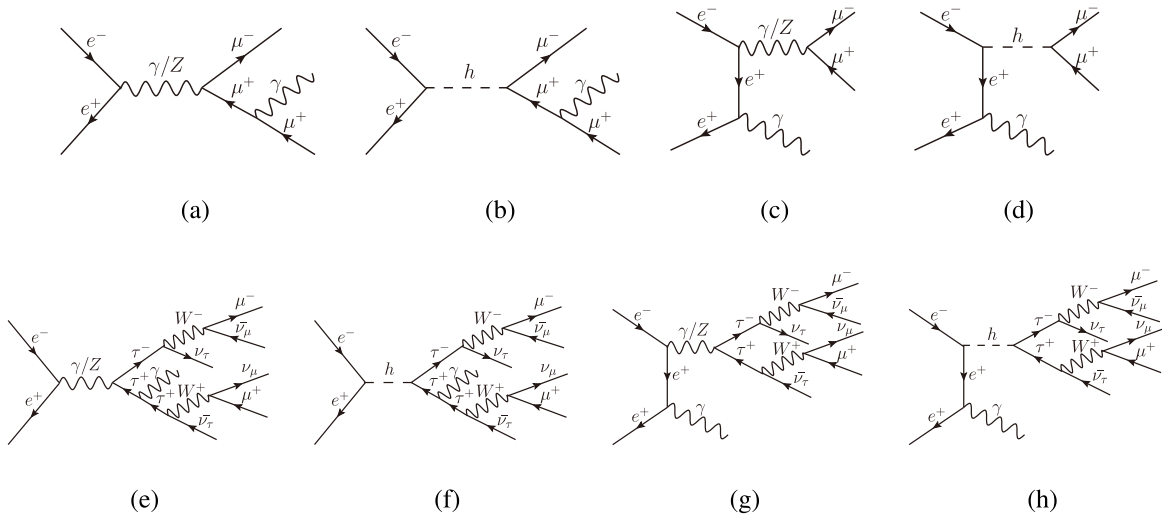
Fig. 6. The Feynman diagrams correspond to the SM background processes e^+e^- \rightarrow \mu^+\mu^-\gamma (a-d), e^+e^- \rightarrow \tau^+\tau^-\gamma , in which one tau lepton radiates a photon before decaying into \mu\nu\bar{\nu} (e,f), and e^+e^- \rightarrow \tau^+\tau^-\gamma , in which both tau leptons subsequently decay into \mu\nu\bar{\nu} (g,h).
