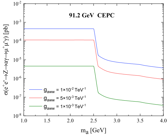
Fig. 5. (color online) Production cross sections for the \mu^+\mu^-\gamma signal as functions of the ALP mass m_a for several representative values of the coupling g_{aWW} at the CEPC operating at 91.2 GeV.
