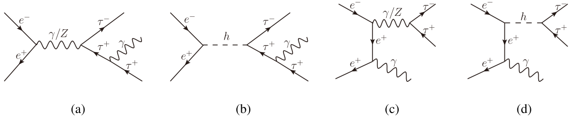
Fig. 9. Feynman diagrams for the SM background process e^+e^- \rightarrow \tau^+\tau^-\gamma .
