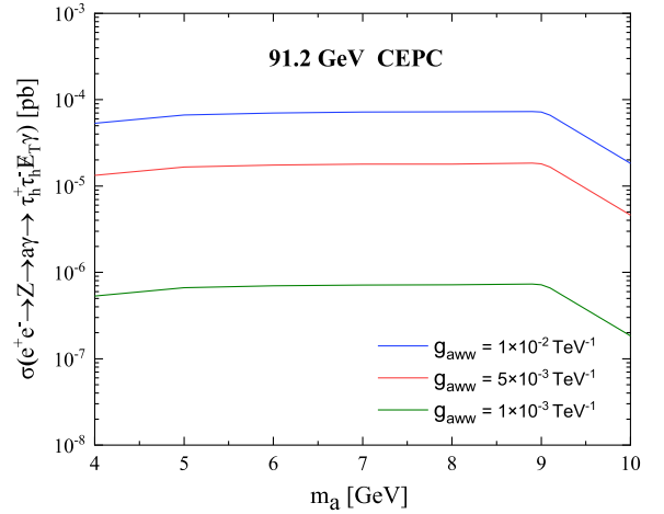
Fig. 8. (color online) Same as Fig. 5, but for the \tau_h^+\tau_h^-\mathbb{E}_T\gamma signal.
