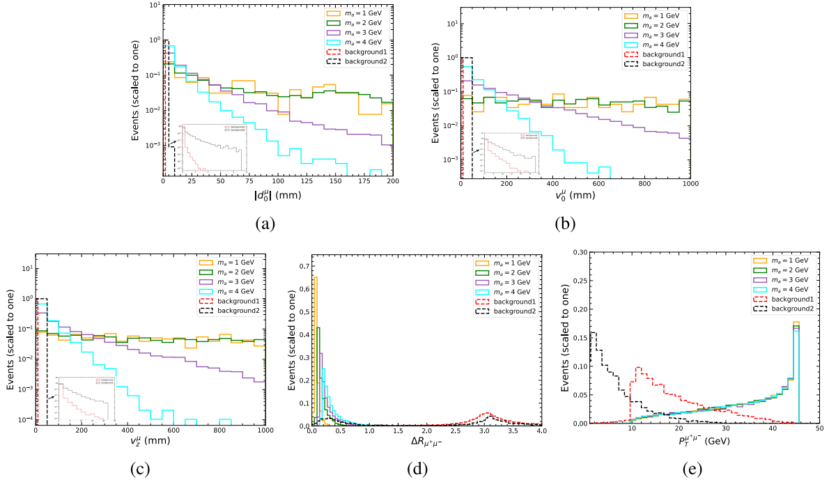
Fig. 7. (color online) The normalized distributions of |d_0^\mu| , v_0^\mu , v_z^\mu , \Delta R_{\mu^+\mu^-} , and P_T^{\mu^+\mu^-} for the \mu^+\mu^-\gamma signal at selected ALP mass benchmark points with g_{aWW} = 5 \times 10^{-3} \text{ TeV}^{-1} , as well as for the SM background, at the CEPC operating at 91.2 GeV with \mathcal{L} = 100 \text{ ab}^{-1} .
