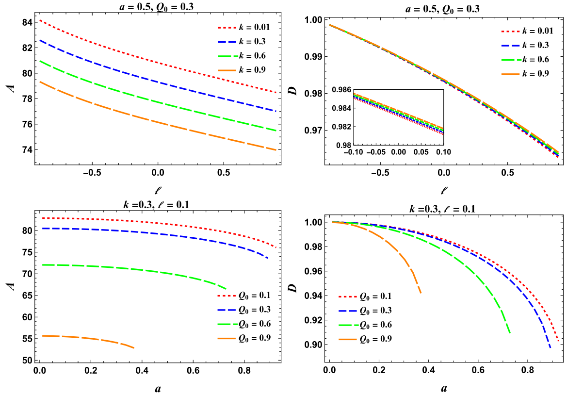
Fig. 8. (color online) Variations of the shadow area A and the oblateness D for a KN-like black hole in Bumblebee gravity surrounded by plasma. The fixed parameters are set to a = 0.5 , Q_0 = 0.3 (upper row), and k = 0.3 , \ell = 0.1 (bottom row).
