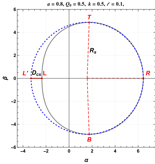
Fig. 6. (color online) Illustration of the shadow observables defined by the reference circle method. The solid black curve represents the black hole shadow, and the dashed blue curve denotes the reference circle. This circle is constructed to pass through three characteristic points: the top ( T ), bottom ( B ), and rightmost ( R ) points of the shadow. Here, L and L' denote the left endpoints of the shadow and the reference circle, respectively. The parameter D_{cs} is defined as D_{cs} \equiv \alpha_{L'} - \alpha_L .
