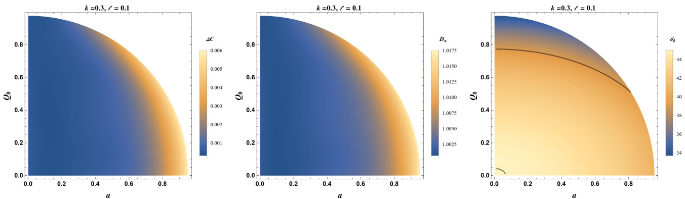
Fig. 10. (color online) Density plots of the circular deviation \Delta C , axial ratio D_x , and angular diameter \theta_d in the (a, Q_0) parameter plane for \theta_0 = 17^\circ . The parameter plane includes only values for which an event horizon exists.
