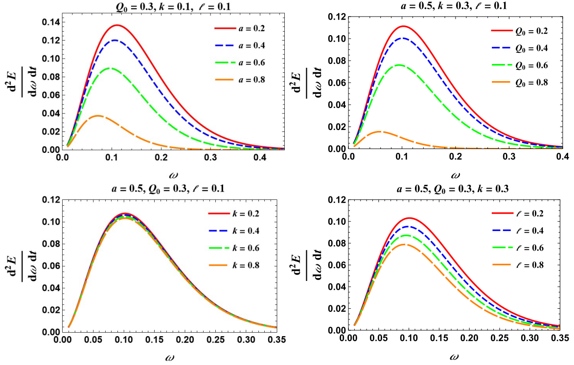
Fig. 9. (color online) High-frequency energy emission rate as a function of frequency \omega for different values of the physical parameters (a, Q_0, k, \ell) .
