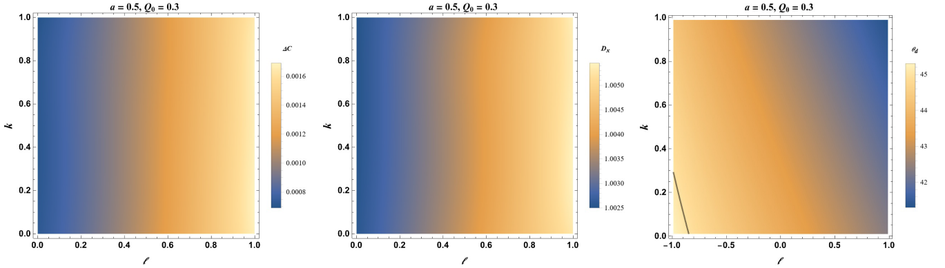
Fig. 11. (color online) Density plots of the circular deviation \Delta C , axial ratio D_x , and angular diameter \theta_d in the (\ell, k) parameter plane for \theta_0 = 17^\circ . The parameter plane includes only parameter values for which an event horizon exists.
