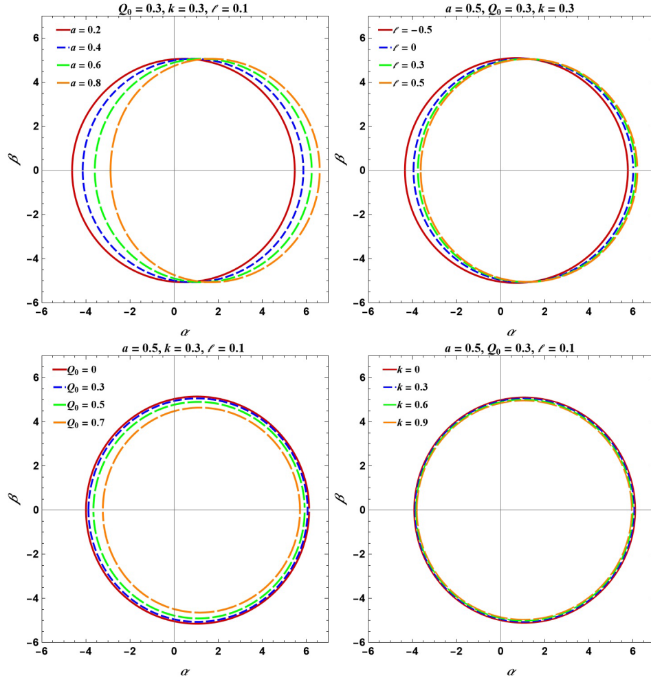
Fig. 5. (color online) Shadows of the KN-like black hole in Bumblebee gravity surrounded by plasma, illustrating the independent effects of variations in the parameters a , \ell , Q_0 , and k .
