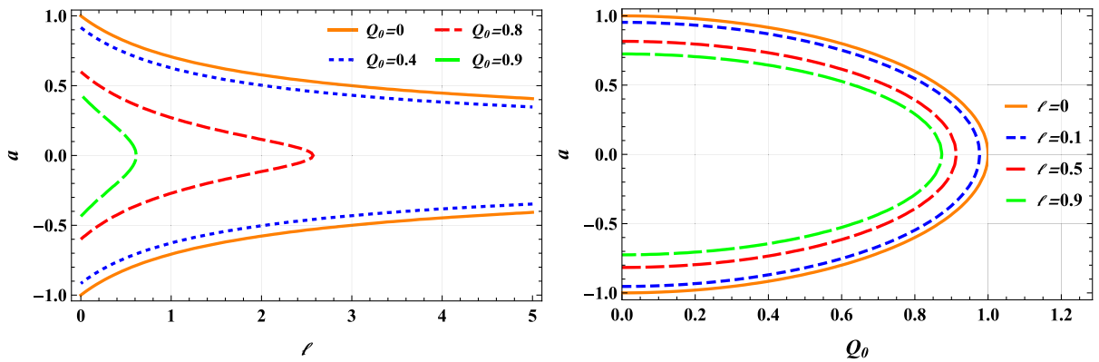
Fig. 1. (color online) Parameter space of the Bumblebee black hole ( M = 1 ). The boundary curves represent the extremal black hole condition, corresponding to the degenerate roots of the radial metric function. The region enclosed by the curves denotes the parameter space in which an event horizon exists, whereas the exterior region corresponds to naked singularities.
