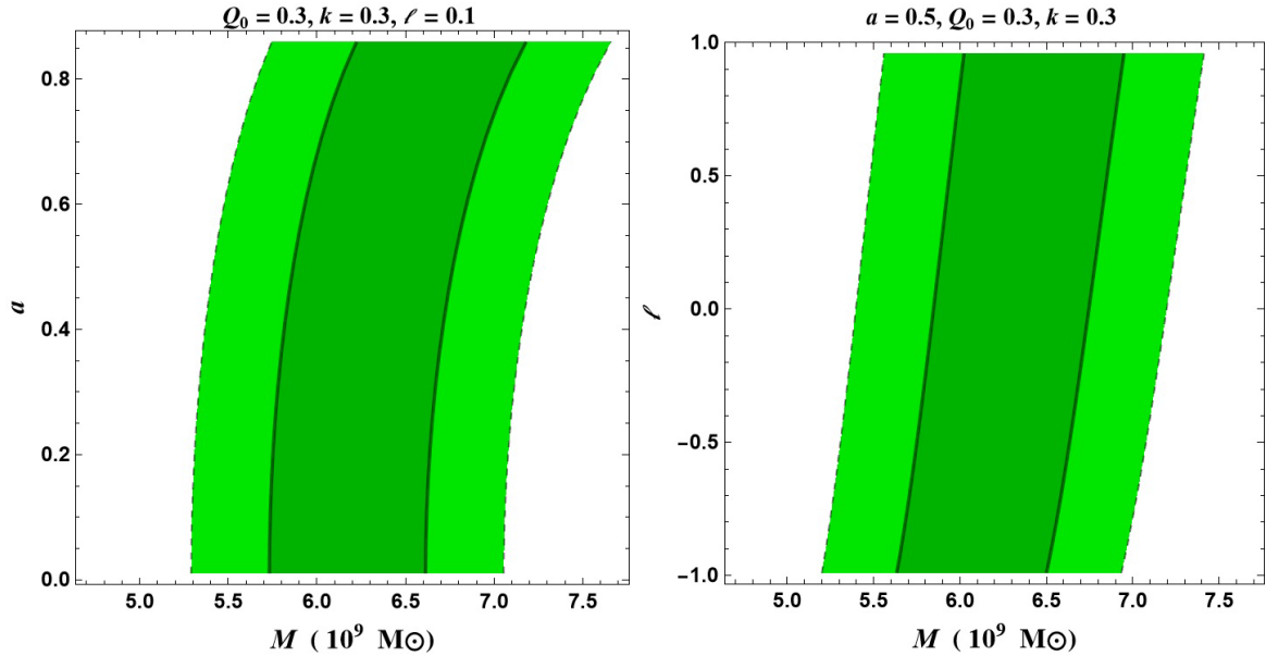
Fig. 12. (color online) Constraints on the parameter a , \ell , and the estimated M87* black hole mass M (\times 10^9 M_\odot) obtained using the M87* shadow angular size within 1\sigma (dark green region) and 2\sigma (light green region).
