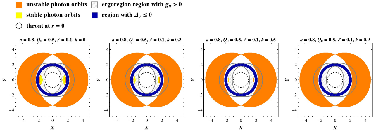
Fig. 3. (color online) Photon regions of the KN-like black hole in Bumblebee gravity surrounded by plasma in the (r, \theta) plane. The parameters are set to a=0.8 , Q_0=0.5 , and \ell=0.1 , with the plasma parameter k varied.
