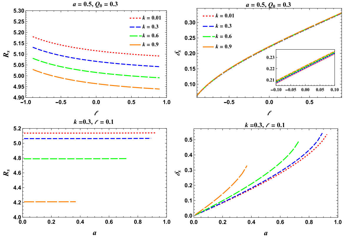
Fig. 7. (color online) Variations in the shadow radius R_s and the distortion parameter \delta_s for a KN-like black hole in Bumblebee gravity surrounded by plasma. The fixed parameters are a = 0.5 , Q_0 = 0.3 in the upper row and k = 0.3 , \ell = 0.1 in the bottom row.
