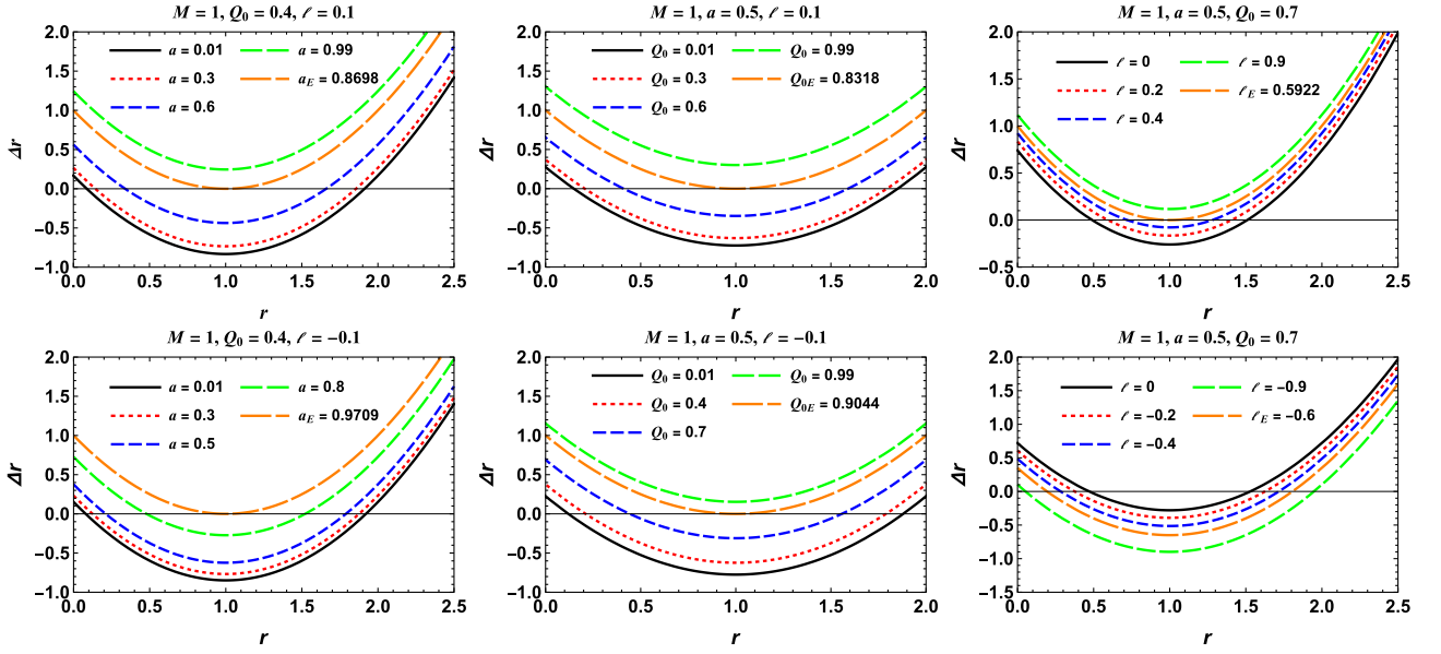
Fig. 2. (color online) Plots of the radial function \Delta_r(r) as a function of r for different parameter combinations ( M = 1 ). The columns, from left to right, show the effects of the spin a , charge Q_0 , and Lorentz-violating parameter \ell , while the upper and lower rows correspond to positive and negative \ell , respectively. The roots of \Delta_r(r) = 0 represent the Cauchy horizon (left) and event horizon (right), and tangency indicates an extremal black hole.
