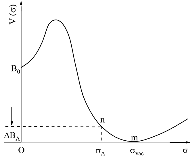
Fig. 1. The potential energy curve V(\sigma) of the scalar field \sigma .
