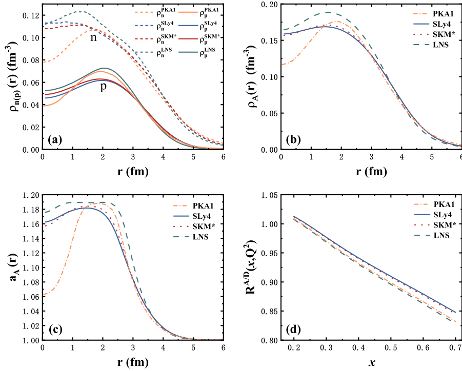
Fig. 3. (color online) The calculated neutron density distribution \rho_n(r) and proton density distribution \rho_p(r) of ^{48}\text{Si} obtained with the PKA1, SLy4, SKM*, and LNS N - N interactions are shown in (a), where the symbols "n" and "p" denote neutrons and protons, respectively. The corresponding nucleon density distribution \rho_A(r) (b), nucleon swelling factor distribution a_A(r) (c), and EMC ratio R^{A/D}(x, Q^2) (d) are also shown. The \rho_n(r) , \rho_p(r) , and \rho_A(r) values for the PKA1 interaction are taken from the RHFB calculation in Ref. [41], whereas those for the SLy4, SKM*, and LNS interactions are obtained from our SHFB calculations.
