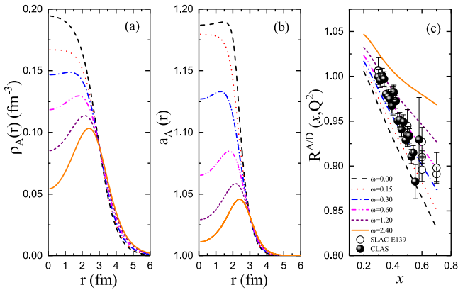
Fig. 2. (color online) The nucleon density distributions \rho_A(r) (a), the corresponding nucleon swelling factor distributions a_A(r) (b), and the computed EMC ratios R^{A/D}(x, Q^2) (c) for ^{27}\text{Al} as functions of r for different \omega values. The open and solid circles represent the experimental data from the SLAC-E139 [21] and CLAS [28] collaborations, respectively.
