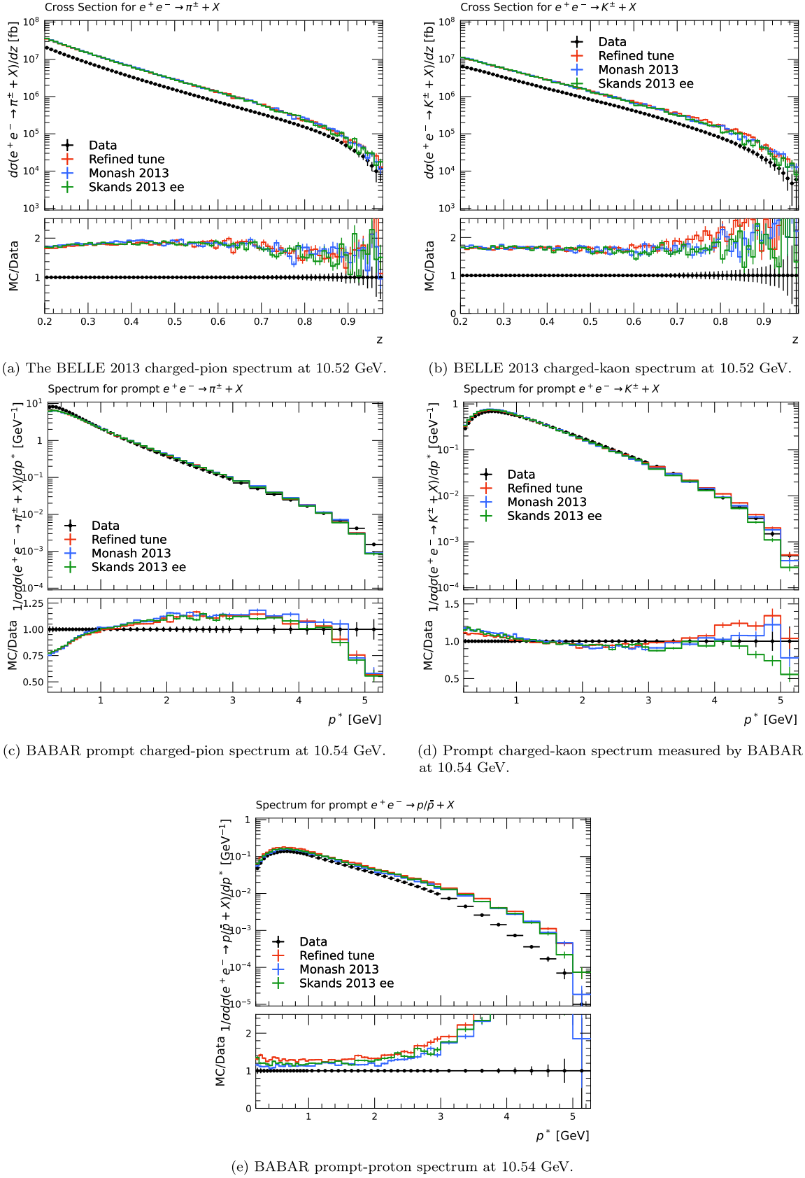
Fig. 1. (color online) In the low-energy charged-hadron sector, the selected refined tune remains the best description of the BELLE 2013 charged-hadron spectra, although the nearby BABAR sample is still described more accurately by the Skands reference.
