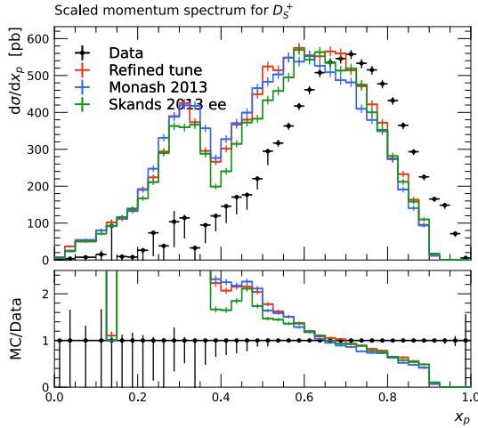
(a) D_s^+ scaled-momentum spectrum.
