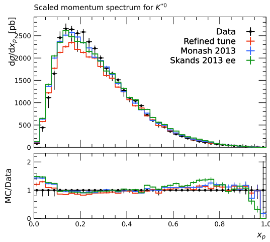
(c) K^{*0} scaled-momentum spectrum.
