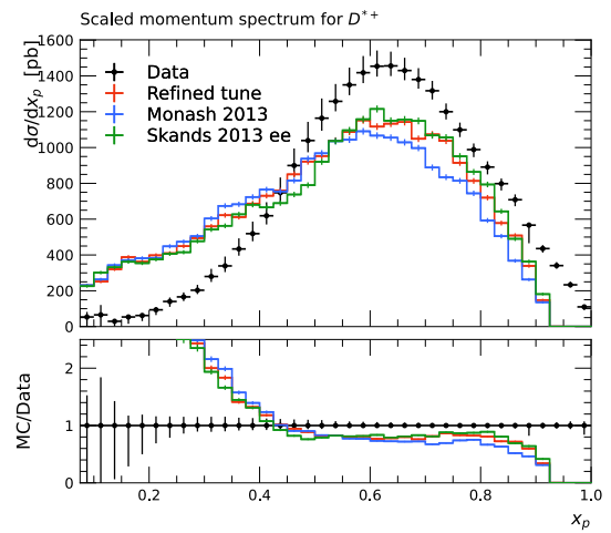
(b) D^{*+} scaled-momentum spectrum.
