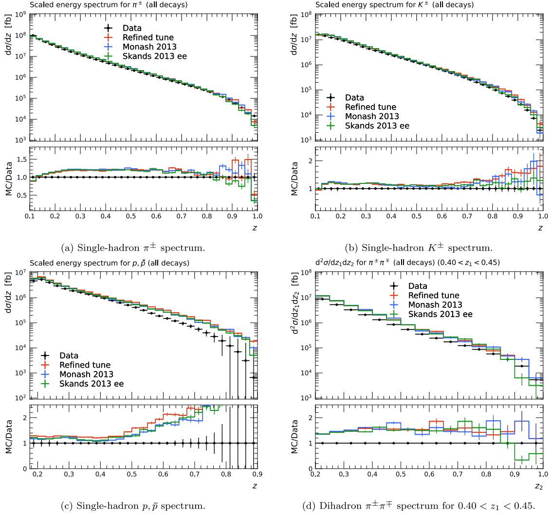
Fig. 2. (color online) Selected BELLE 2020 single- and dihadron spectra. The differences among the three tune curves are modest; however, BELLE 2020 provides most of the common bins and therefore largely determines the bin-weighted ranking.
