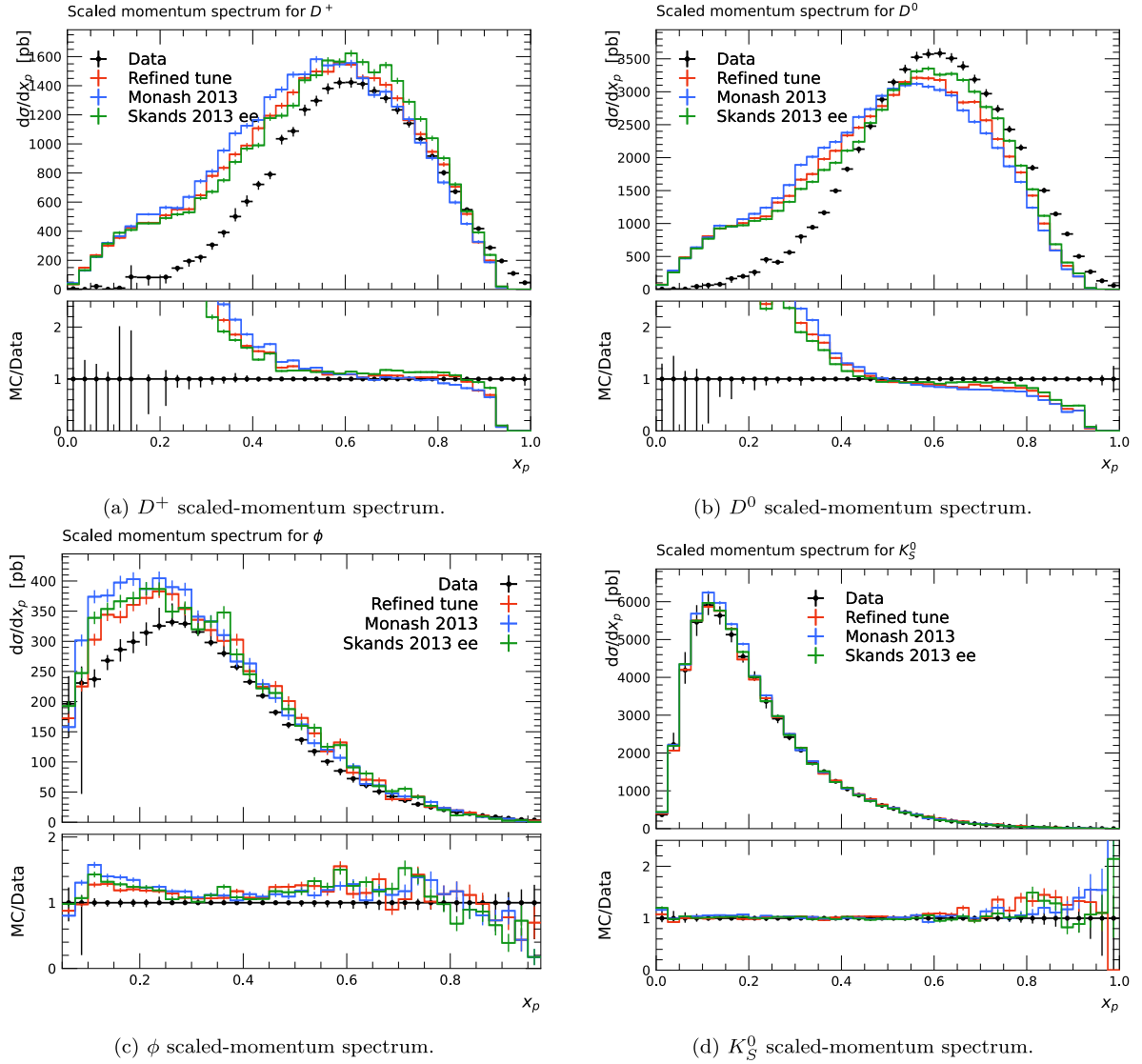
Fig.3. (coloronline) Selected BELLE 2025 meson spectra. The selected tune agrees more closely with the data than Monash in some channels, although Skands achieves the lowest aggregate BELLE 2025 score.
