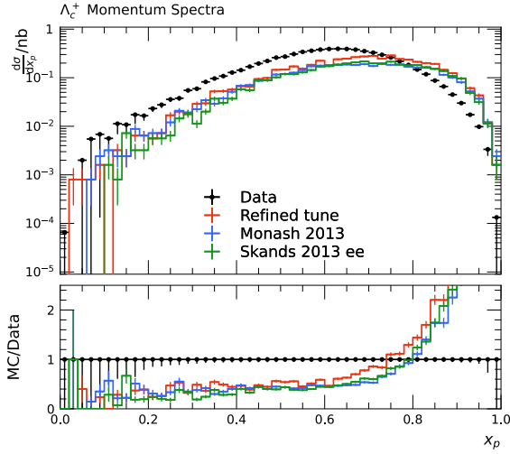
(c) \Lambda_c^+ momentum spectrum.
