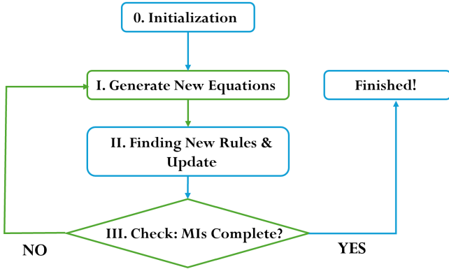
Fig. 1. (color online) The iterative structure of the reduction algorithm.
