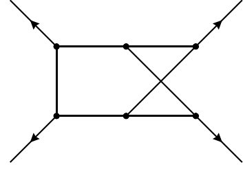
Fig. 4. The two-loop non-planar double-box diagram.
