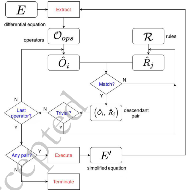
Fig. 2. (color online) Flowchart of the simplification.
