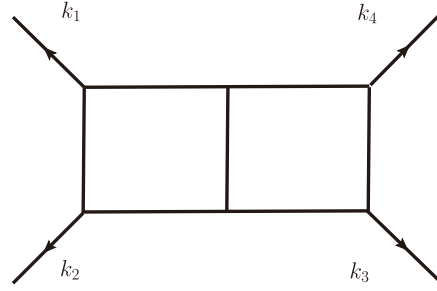
Fig. 3. The two-loop planar double-box diagram.
