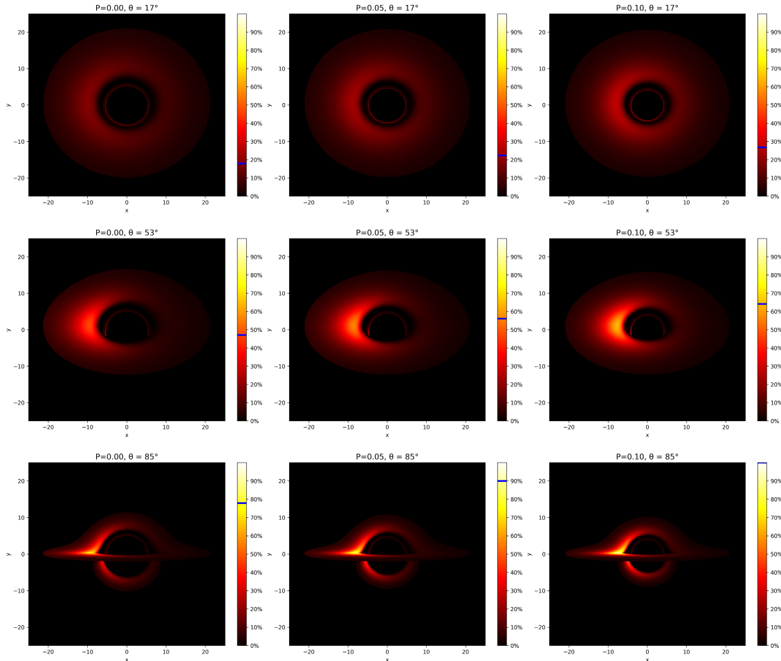
Fig. 8. (color online) Distribution of the observed flux F_{\text{obs}} in the direct and secondary images of a self-dual BH in LQG for inclination angles of 17^\circ , 53^\circ , and 85^\circ .
