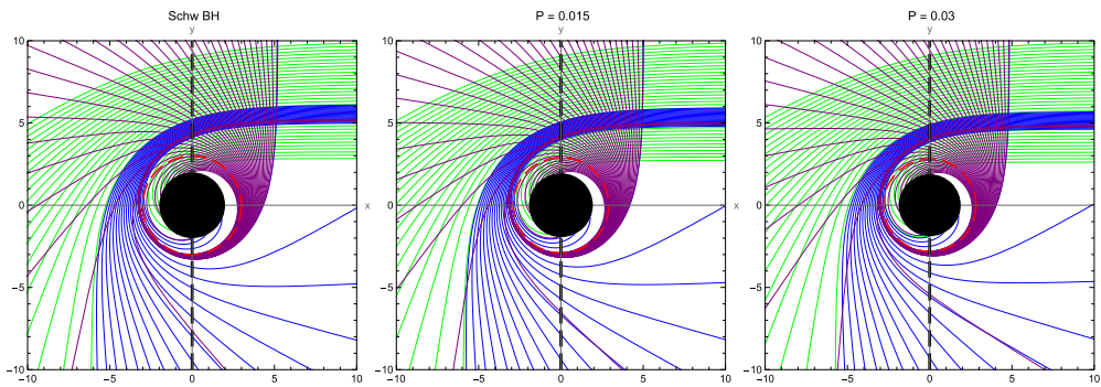
Fig. 2. (color online) Photon trajectories as a function of b for self-dual black holes in LQG. The green, blue, and purple curves correspond to 1/4 < \eta < 3/4 , 3/4 < \eta < 5/4 , and \eta > 5/4 , respectively. The red dashed ring denotes the photon sphere.
