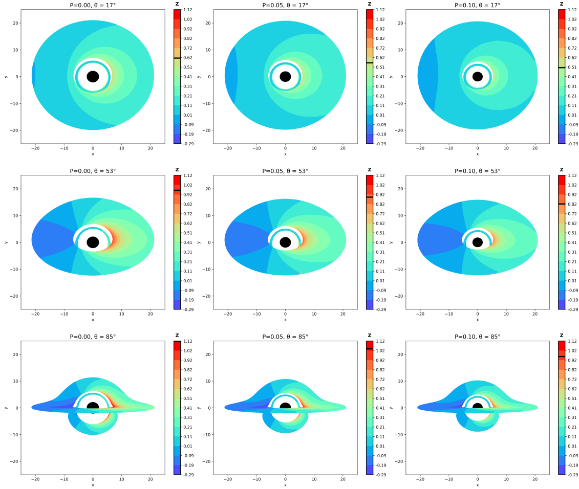
Fig. 9. (color online) The distributions of the redshift factor z for the direct and secondary images of a self-dual BH in LQG are shown for inclination angles of 17^\circ , 53^\circ , and 85^\circ .
