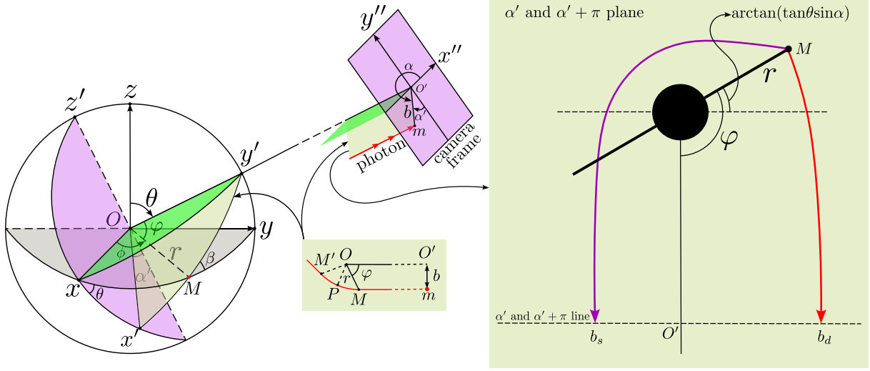
Fig. 4. (color online) Schematic representation of the coordinate system used to construct the image of the accretion disk.
