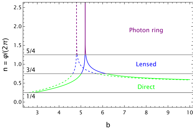
Fig. 3. (color online) The plot shows the number of photon orbits, \eta , as a function of the impact parameter, b . The solid curve corresponds to the Schwarzschild BH, whereas the dashed curve represents the case with P = 0.03 .
