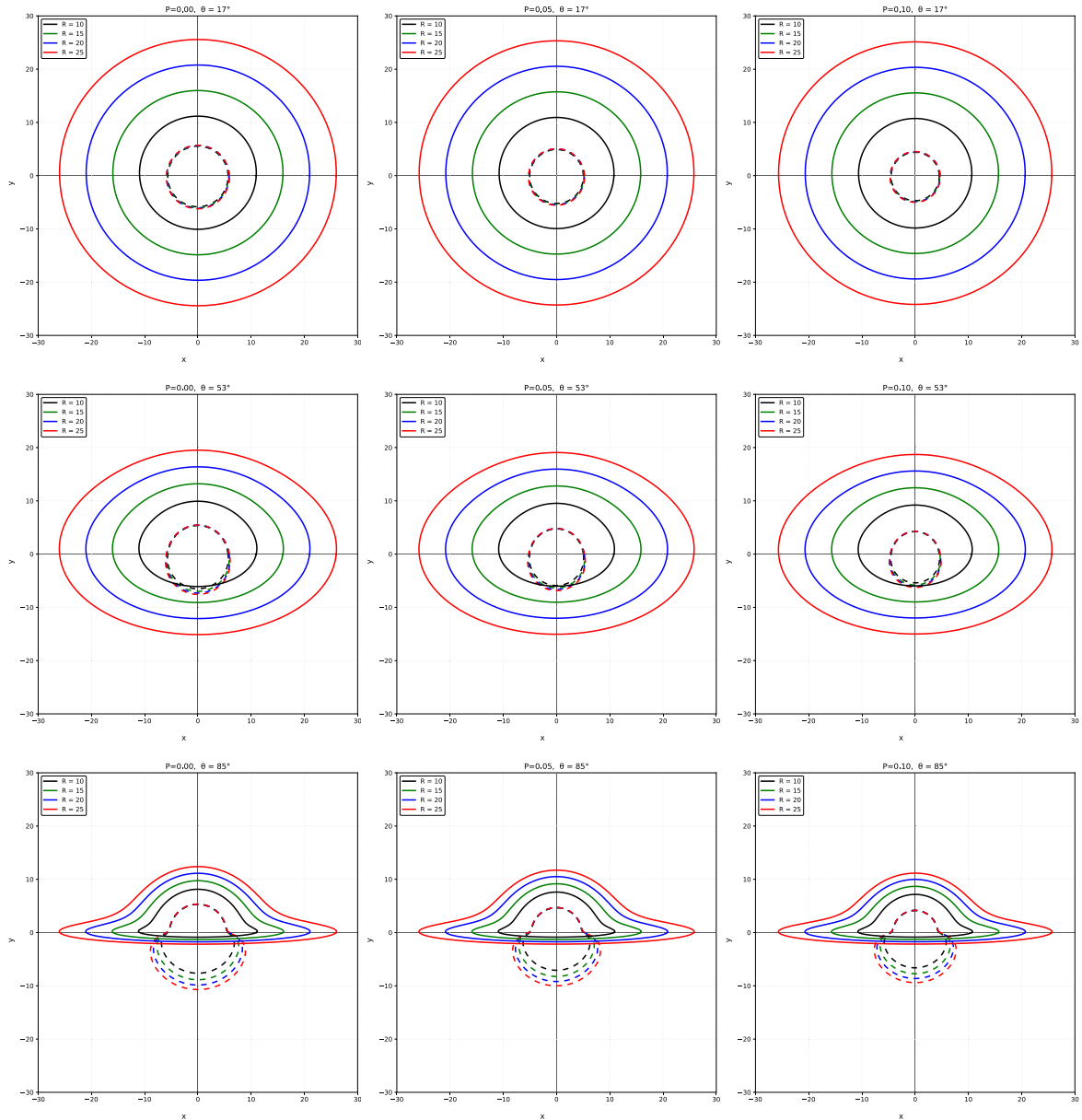
Fig. 6. (color online) Direct and secondary images of the thin accretion disk around a self-dual BH in LQG. From top to bottom, the rows represent inclination angles of 17^\circ , 53^\circ , and 85^\circ ; from left to right, the columns correspond to P values of 0.0 , 0.05 , and 0.10 .
