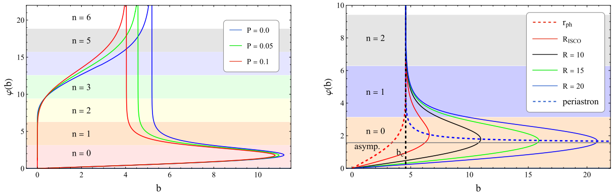
Fig. 5. (color online) Image formation diagrams for various values of the quantum correction parameter P at fixed radius R = 10 (left panel) and for various values of the radius R at fixed P = 0.05 (right panel). The innermost stable circular orbit is at R_{\text{ISCO}} = 5.455 , corresponding to the solid red curve.
