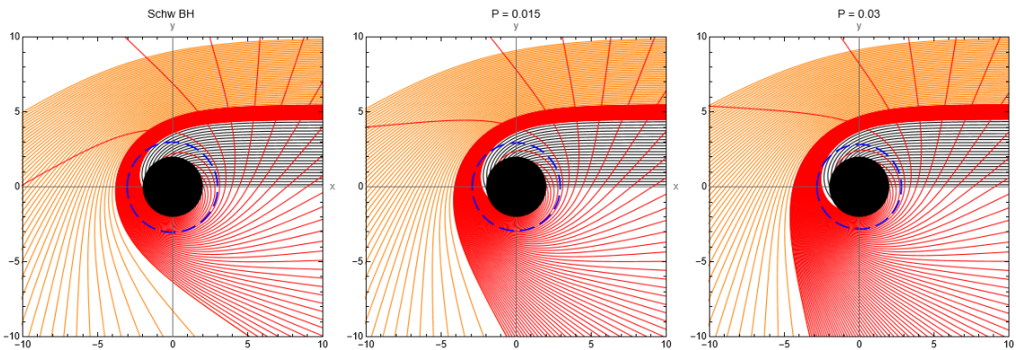
Fig. 1. (color online) Photon trajectories are shown in separate plots for different values of P . In all plots, the colors are assigned as follows: black for 0 < b \leq 4.5 , red for 4.5 < b \leq 5.5 , and orange for b > 5.5 . The blue dashed ring represents the photon sphere.
