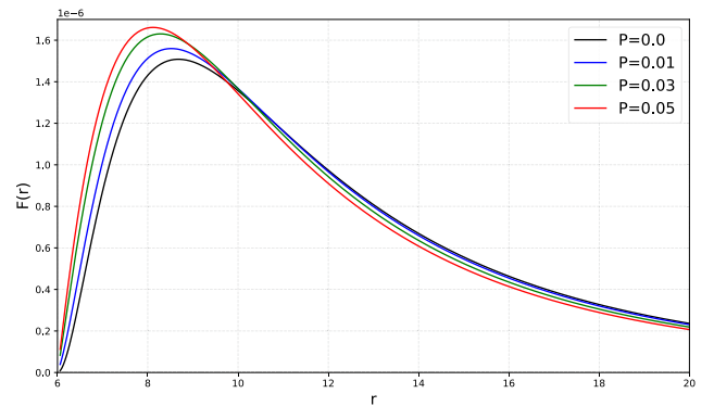
Fig. 7. (color online) Energy flux F(r) as a function of the radius r for different values of the quantum correction parameter P .
