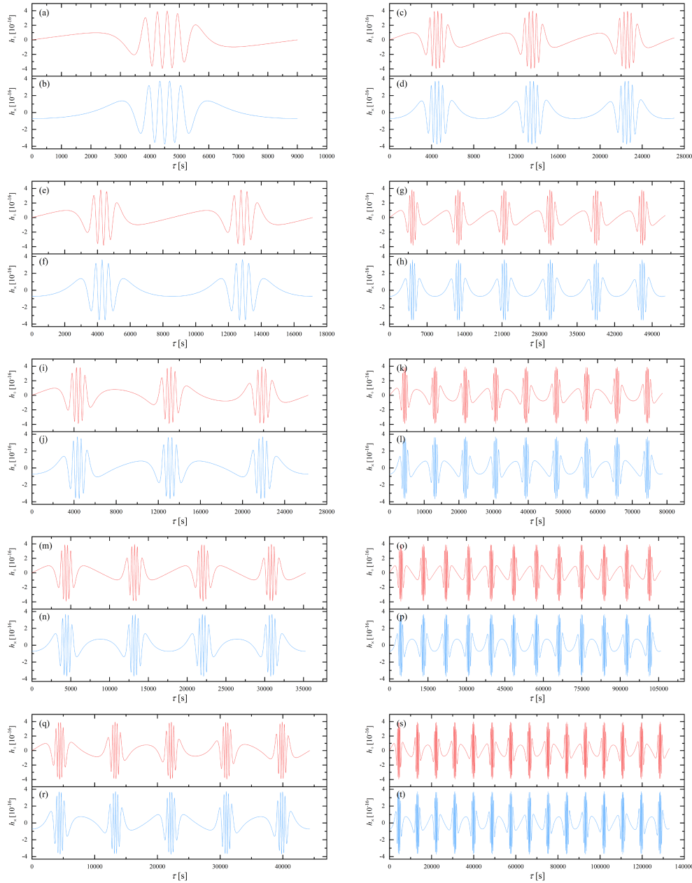
Fig. 6. (color online) Time-domain gravitational wave signals of rational orbits (left column) and irrational orbits (right column). From top to bottom, z sequentially increases from 1 to 5. In each panel, red and blue correspond to the h_+ and h_x polarization states, respectively. The left column shows that within one orbital period, the number of high-frequency oscillations in the gravitational wave signal is consistent with the number of orbital leaves.
