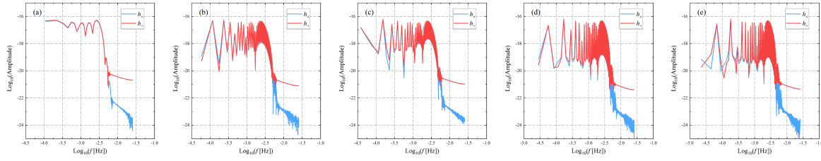
Fig. 7. (color online) Frequency-domain information obtained via the fast Fourier transform from the time-domain gravitational wave signals of the rational orbits in Fig. 6. From left to right, the number of orbital leaves z sequentially increases from 1 to 5. It can be observed that the frequency-domain amplitudes of the gravitational waves are relatively strong below 0.01 Hz. Meanwhile, it is almost impossible to establish a connection between the frequency-domain gravitational wave signals and the orbital configurations.
