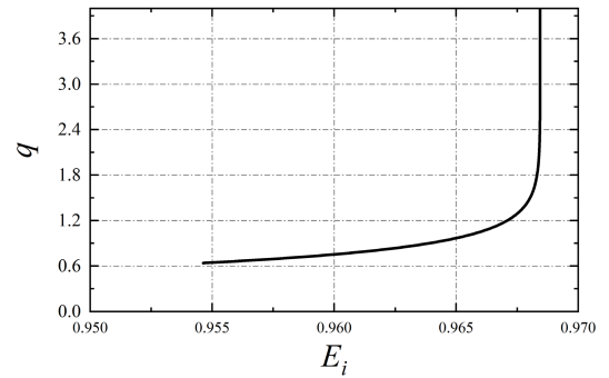
Fig. 4. Rational number q as a function of the specific energy E_i . It is clear that q exhibits a lower limit since E_i has a minimum value.
