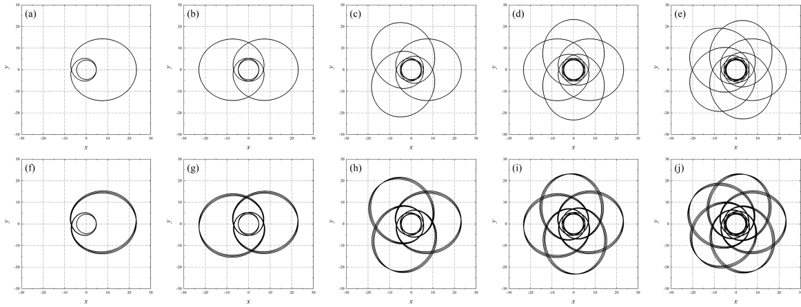
Fig. 5. Rational orbits (first row) and irrational orbits (second row) corresponding to different orbital configurations. From left to right, the numbers of orbital leaves are z = 1, 2, 3, 4 , and 5 , and we have \nu = z - 1 for z > 1 , while \nu = 1 for z = 1 . The irrational orbits are obtained by adding 1/100z to q . Here, we fix w = 1 . The simulated proper time for rational orbits is exactly one orbital period T_q , whereas the simulation time for irrational orbits is three times T_q .
