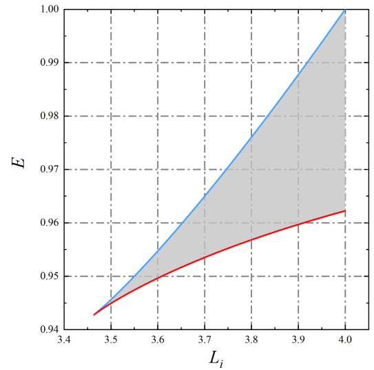
Fig. 3. (color online) Evolution of the maximum specific energy E_{\max} and the minimum specific energy E_{\min} corresponding to stable orbits with respect to the orbital angular momentum L_i . The shaded region between the two curves represents the parameter space where stable orbits exist.
