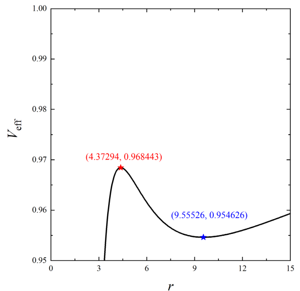
Fig. 1. (color online) Effective potential V_{\text{eff}} as a function of r in the case of L_i = 3.7321 . The red and blue star markers correspond to the maximum and minimum points, respectively, representing the locations of the unstable circular orbit and the stable circular orbit.
