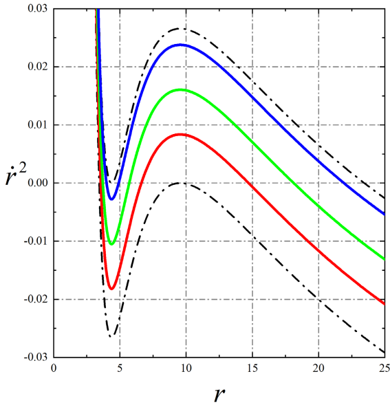
Fig. 2. (color online) \dot{r}^2 as a function of r . The red, green, and blue solid lines correspond to E_1 = 0.959 , E_2 = 0.963 , and E_3 = 0.967 respectively. The upper and lower dash-dotted lines correspond to E_{\max} and E_{\min} , respectively. It can be observed that the red, blue, and green lines intersect the line \dot{r}^2 = 0 three times, indicating the existence of stable orbits, and the two larger roots correspond to the apastron and periastron of the orbits. In contrast, the two dash-dotted lines intersect the line \dot{r}^2 = 0 only twice, corresponding to circular orbits.
