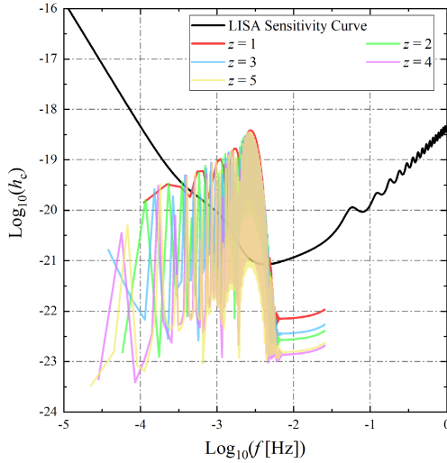
Fig. 8. (color online) Comparison between the characteristic strains of gravitational waves for different orbital configurations and the LISA sensitivity curve (black). It can be found that the characteristic strains of all the displayed orbital configurations have portions exceeding the LISA sensitivity curve, and these correspond to the mHz frequency window. This demonstrates that the gravitational radiation from the rational orbits investigated in this paper has the potential to be observed in the future.
