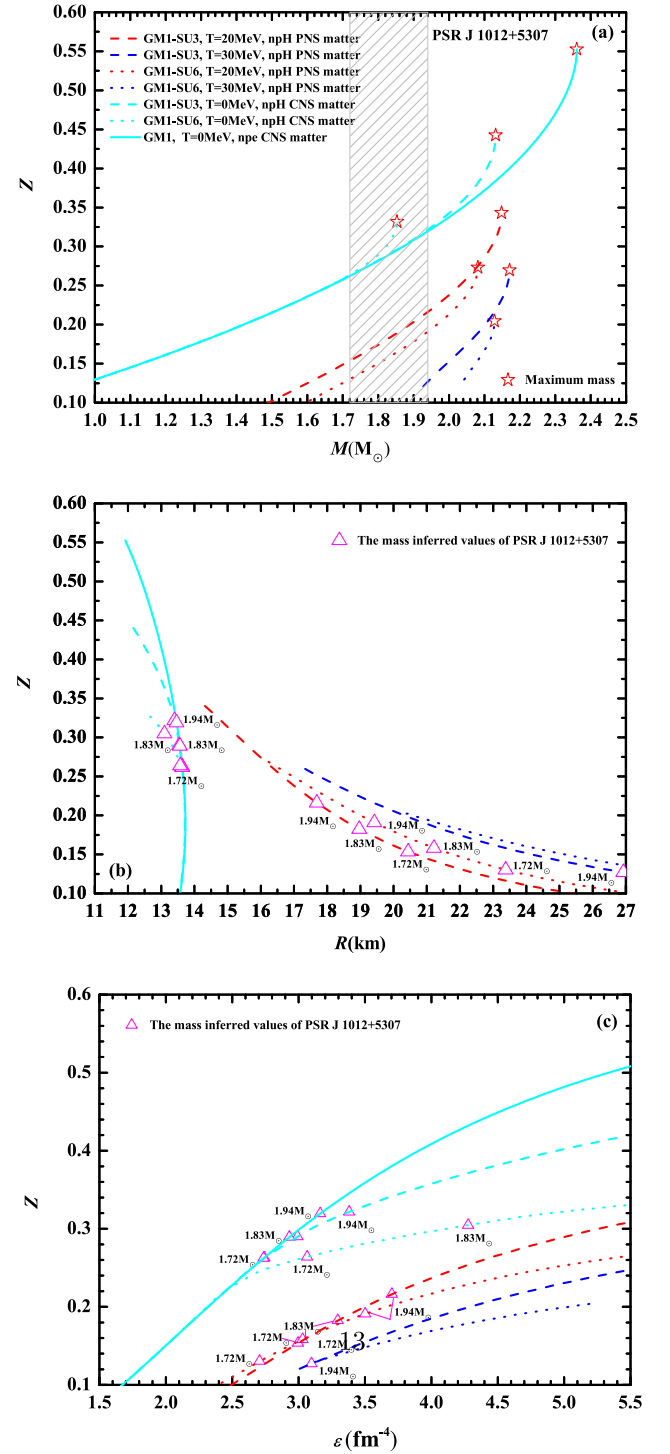
Fig. 3. (color online) Gravitational redshift of PNSs and CNSs. (a) Gravitational redshift as a function of mass. (b) Gravitational redshift as a function of radius. (c) Gravitational redshift as a function of central energy density.
