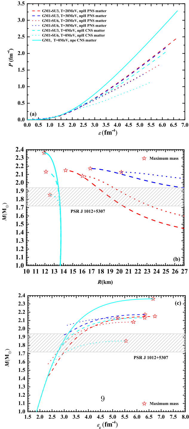
Fig. 1. (color online) (a) EOSs of PNSs and CNSs. (b) Mass-radius relations. (c) Mass-central energy density relations. Cyan lines show the CNS results at T = 0 MeV. Solid lines correspond to npe matter, whereas dashed and dotted lines correspond to npeH matter with SU(3) flavor and SU(6) spin-flavor symmetries, respectively. Red and blue lines show the PNS results at T = 20 MeV (red) and T = 30 MeV (blue) under SU(3) (dashed) and SU(6) (dotted) symmetries, respectively. Red stars indicate the maximum masses for each configuration. This notation is used consistently in subsequent figures.
