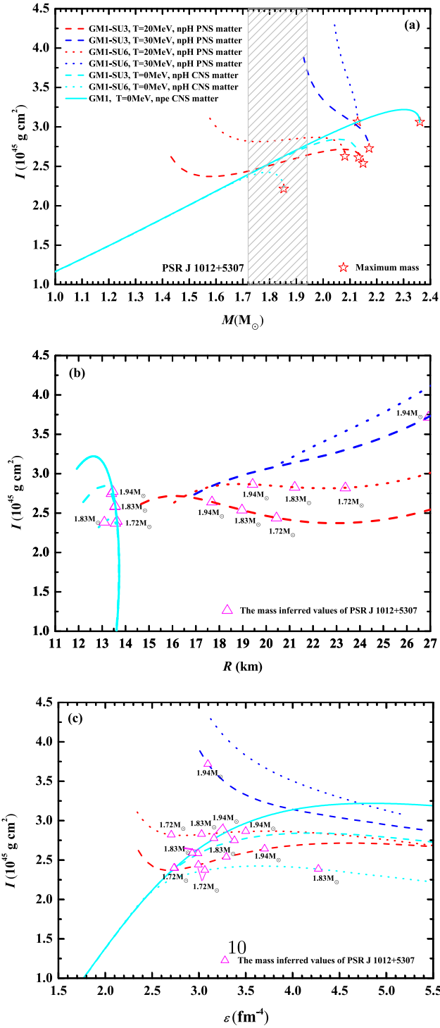
Fig. 2. (color online) Moment of inertia of PNSs and CNSs. (a) Moment of inertia as a function of mass. (b) Moment of inertia as a function of radius. (c) Moment of inertia as a function of central energy density. Pink triangles denote mass measurements of PSR J1012+5307. This notation is used consistently in subsequent figures.
