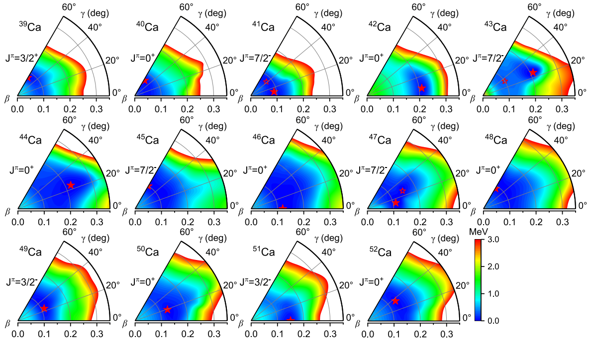
Fig. 2. (color online) This figure is analogous to Fig. 1(c), but it pertains to the calcium isotopes ranging from ^{39}\text{Ca} to ^{52}\text{Ca} . The red solid stars represent the locations of the global minima, whereas the red open stars indicate the associated secondary local minima.
