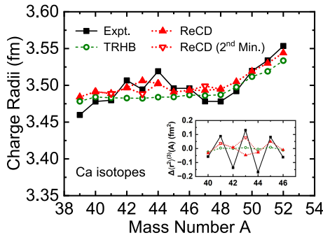
Fig. 4. (color online) Charge radii of calcium isotopes calculated within the ReCD framework (red solid triangles) are compared with results from TRHB mean-field calculations (green open circles) and available experimental data (black solid squares) [23]. The red open triangles represent the charge radii derived from the many-body wavefunctions associated with the secondary local minima shown in Fig. 2. The inset displays the corresponding odd-even staggering factor, \Delta\langle r^2 \rangle^{(3)}(A) , extracted using the three-point formula for calcium isotopes with mass numbers ranging from 40 to 46; see the text for details.
