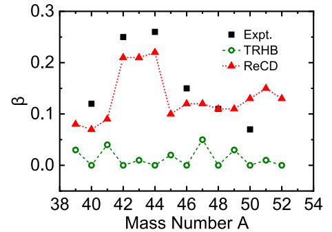
Fig. 3. (color online) The quadrupole deformation parameter \beta at the energy minima positions on the PESs for ^{39-52}\text{Ca} , as determined from the ReCD calculations (red solid triangles), is compared with results from TRHB calculations (green open circles) and available experimental data (black solid squares) [62].
