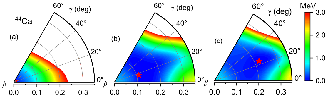
Fig. 1. (color online) Potential energy surfaces (PESs) of ^{44}\text{Ca} are depicted in the plane defined by the axially symmetric quadrupole deformation parameter \beta and the triaxial deformation parameter \gamma . (a) The PES of the mean-field states is obtained by solving the TRHB equation. (b) The PES of the 0^+ states is derived after performing angular-momentum projection on the mean-field states. (c) The PES of the 0^+ states is obtained following both angular-momentum projection and configuration mixing, corresponding to the complete ReCD calculation.
