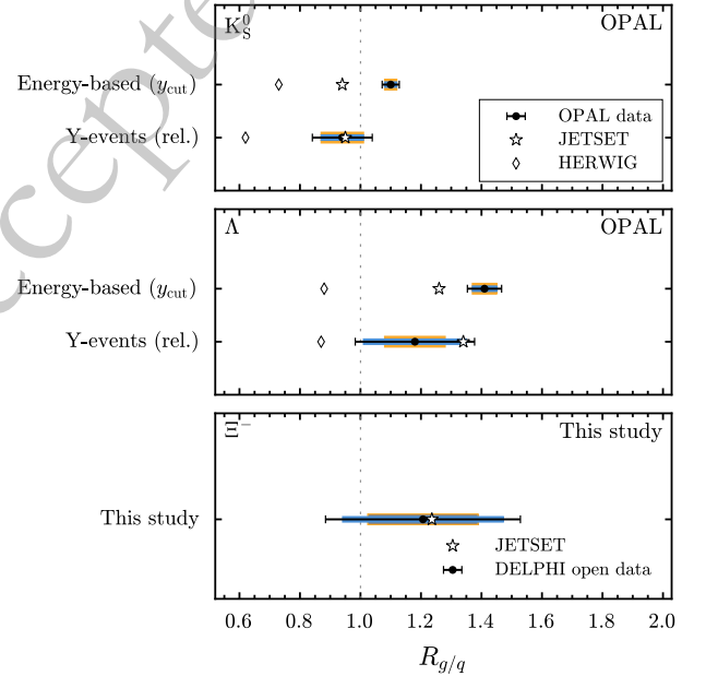
Fig. 4. (color online) Comparison of the gluon-to-quark jet production ratio \mathcal{R}_{g/q} for strange hadrons. The K_S^0 and \Lambda results, along with the JETSET and HERWIG predictions, are obtained from the OPAL measurements [3]. Yellow and blue bands indicate statistical and systematic uncertainties, and black error bars show their quadrature sum.
