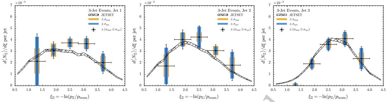
Fig. 3. (color online) Differential \Xi^- production spectra as a function of \xi_{\Xi} = -\ln(p_{\Xi}/p_{\text{beam}}) in Jet 1 , Jet 2 , and Jet 3 of the three-jet events.
