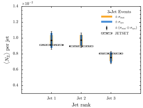
Fig. 2. (color online) Average \Xi^- production per jet in the energy-ranked jets for (left) two- and (right) three-jet events. The measurements are compared with the JETSET prediction.
